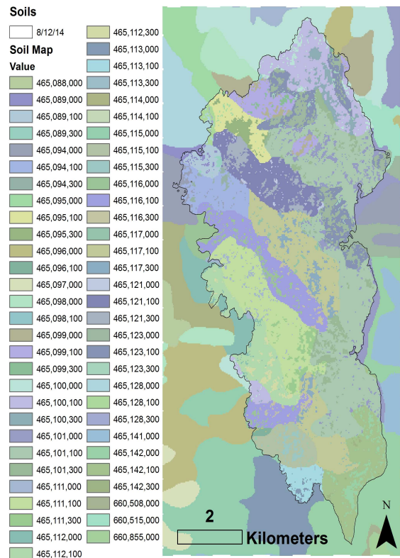
Figure 4. A soils map generated by the database depicting soil files modified by the burned French Fire land cover layer. To facilitate modeling the corresponding WEPP soil parameter and linkage files are also provided by the online database.
