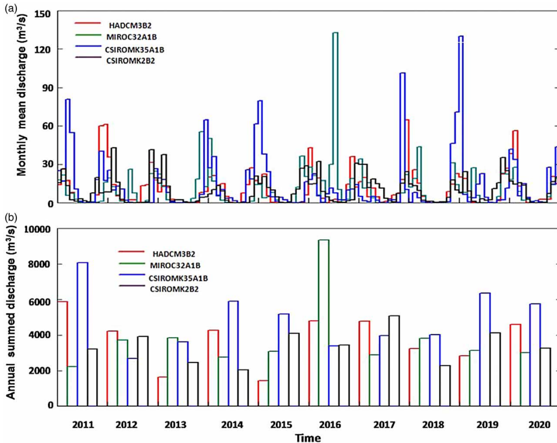
Figure 3 | Simulated and monthly mean (a) and annual sum (b) water discharge for the four simulation scenarios.
