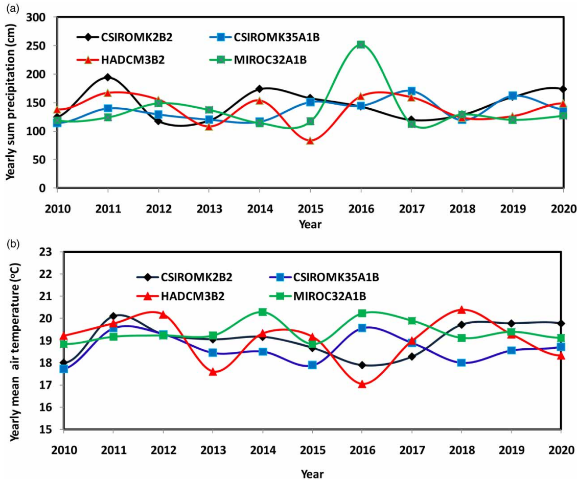
Figure 4 | Annual sum precipitation (a) and mean air temperature (b) for the four future climate change scenarios. Precipitation and air temperature were used as input data for simulations.
