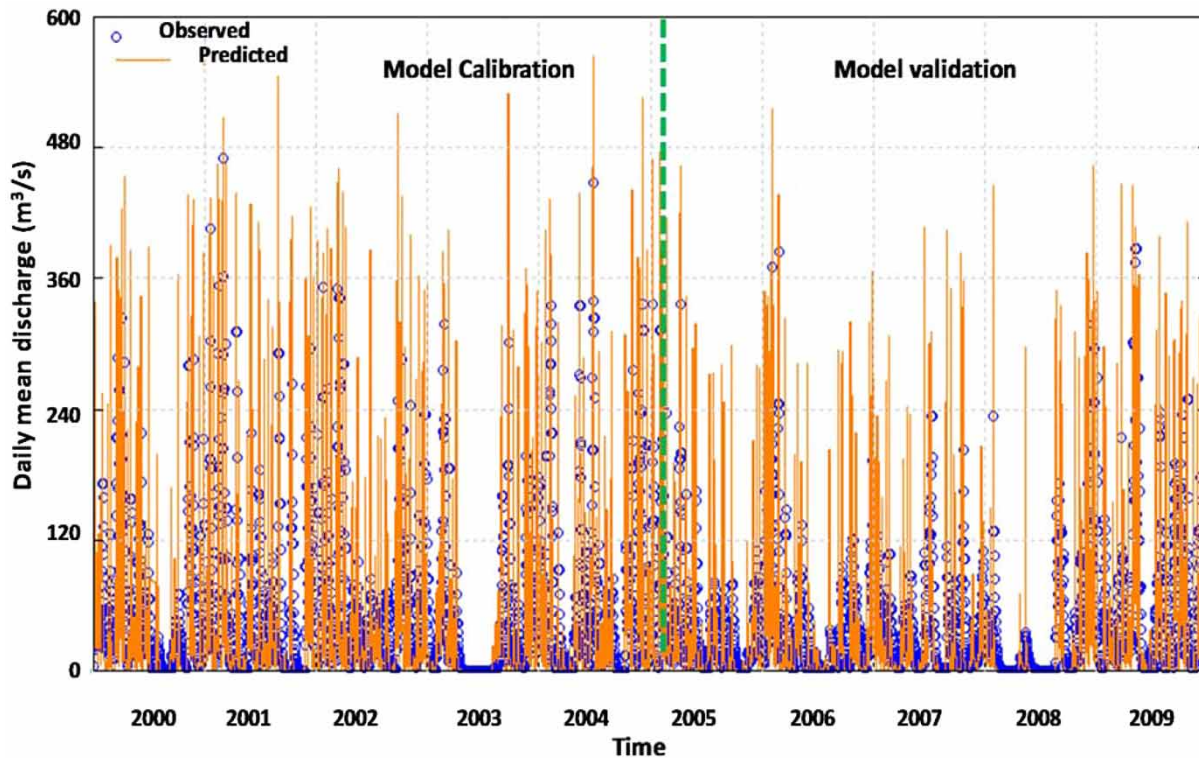
Figure 2 | Comparisons of the observed and predicted daily mean flow rates during model calibration and validation processes.
