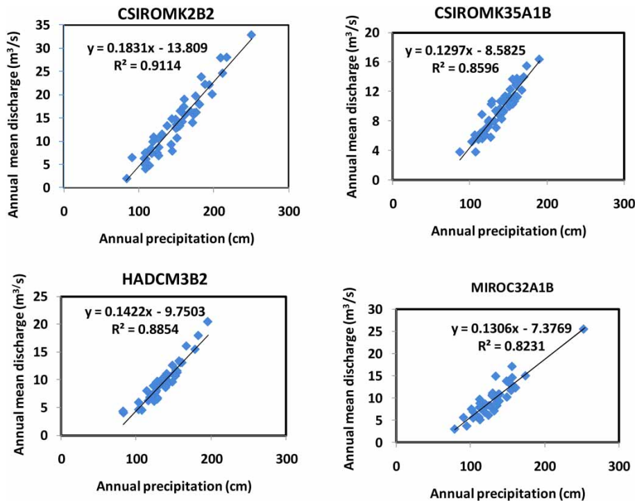
Figure 5 | Relationships of annual precipitation to annual mean water discharge among the four simulation scenarios.
