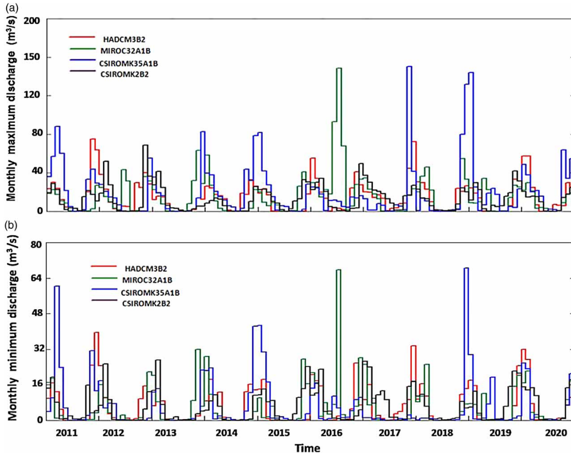
Figure 6 | Simulated monthly maximum (a) and minimum (b) water discharge among the four simulation scenarios.
