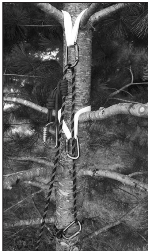
Figure 6a: 4-inch tie-in anchor
