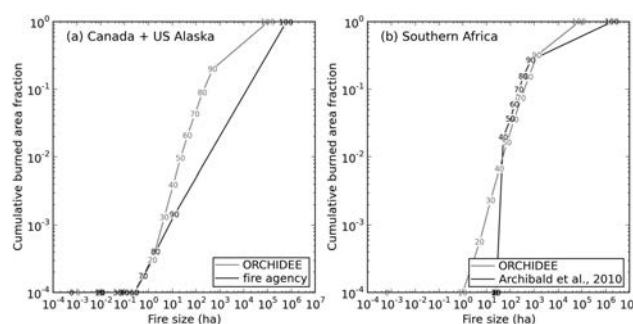
Figure 12. Fire size and the corresponding cumulative fraction of the total burned area by fires below a given fire size for (a) Canada & US Alaska, and (b) southern Africa. Data are shown for a series of equally distanced 10th quantile fire sizes. Numbers in the curves show the location of every 10th quantile fire size from 0th quantile (the minimum fire size) to 100th quantile (the maximum fire size).
