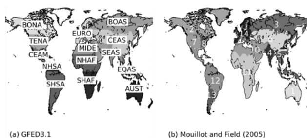
Figure 2. The regional breakup of the globe according to (a) the GFED3.1 data set: BONA, boreal North America; TENA, temperate North America; CEAM, Central America; NHSA, Northern Hemisphere South America; SHSA, Southern Hemisphere South America; EURO, Europe; MIDE, Middle East; NHAf, Northern Hemisphere Africa; SHAF, Southern Hemisphere Africa; BOAS, boreal Asia; CEAS, central Asia; SEAS, Southeast Asia; EQAS, equatorial Asia; AUST, Australia and New Zealand. And (b) Mouillot and Field (2005): (1) Australia and New Zealand; (2) boreal North America; (3) boreal Russia; (4) India; (5) Southeast Asia; (6) central Asia; (7) USA (western Mississippi); (8) USA (eastern Mississippi); (9) East Asia; (10) Middle East and northern Africa; (11) Africa (sub-Saharan); (12) central South America; (13) southern South America; (14) Europe.
