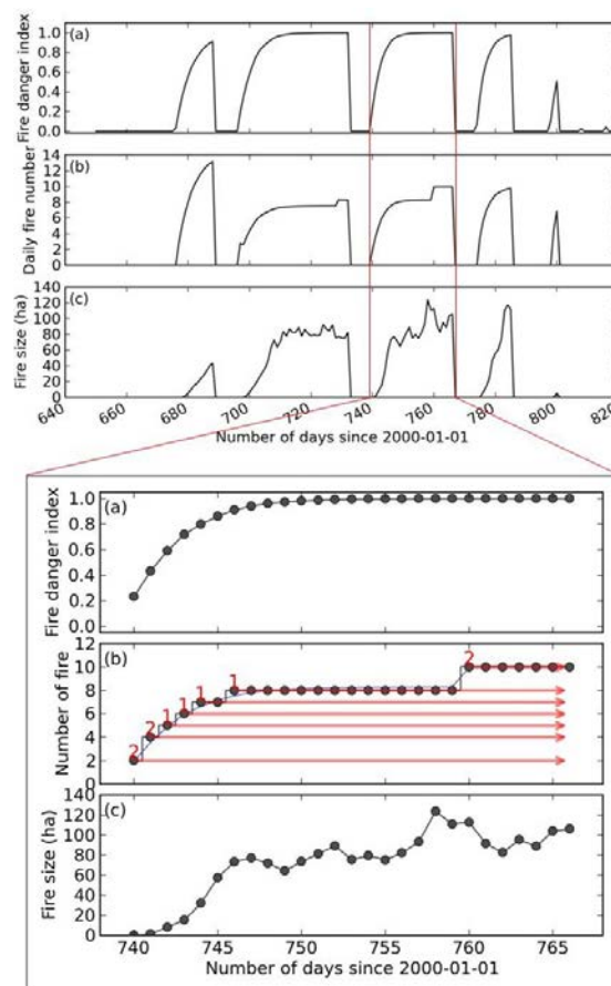
Figure 3. Schematic diagram showing the concatenation of fires within consecutive days into multi-day fire patches. An example is given for a 0.5^\circ grid cell in northern Africa for the fire season from October 2001 to April 2002. Upper panel: fires in different consecutive-day periods as simulated by the model. Lower panel: zooming for the period of Day 740–766 since 1 January 2000. Ten different fire patches were extracted from fires in this period. The number of fire patches and their persistence time were indicated by the numbers and arrows in red in the subplot (b), respectively. Refer to Sect. 2.5.2 for detailed explanations.
