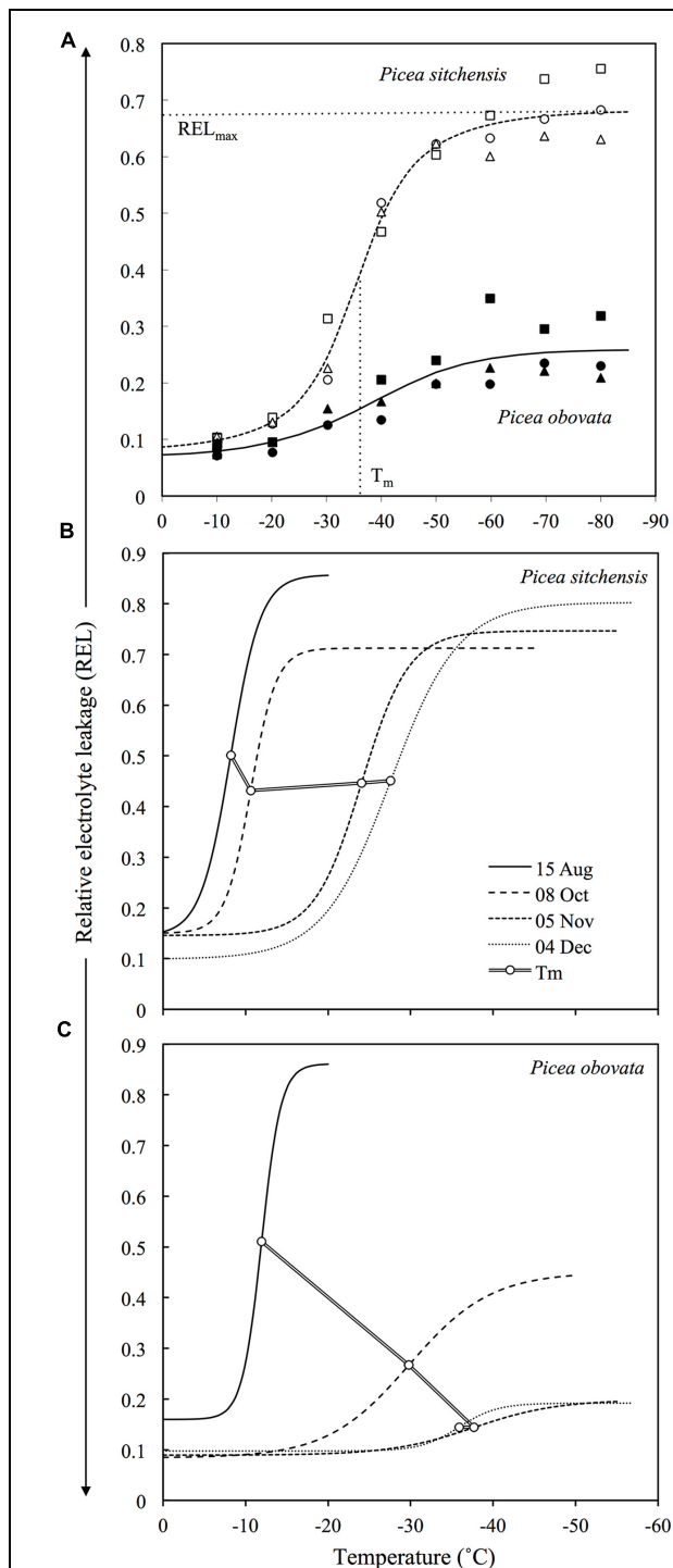
FIGURE 1 | (A) Example of REL data and temperature response curves for fully acclimated needles from MLT and ELT tolerant species ( Picea sitchensis and Picea obovata , respectively). Different symbols represent three different trees for each species. Horizontal and vertical dashed lines show location of the parameters REL_{max} and T_m , respectively for P. sitchensis (adapted from Strimbeck et al., 2007). (B,C) Changes in temperature response curves and T_m during acclimation for P. sitchensis (B) and P. obovata (C) (adapted from Strimbeck et al., 2008).
