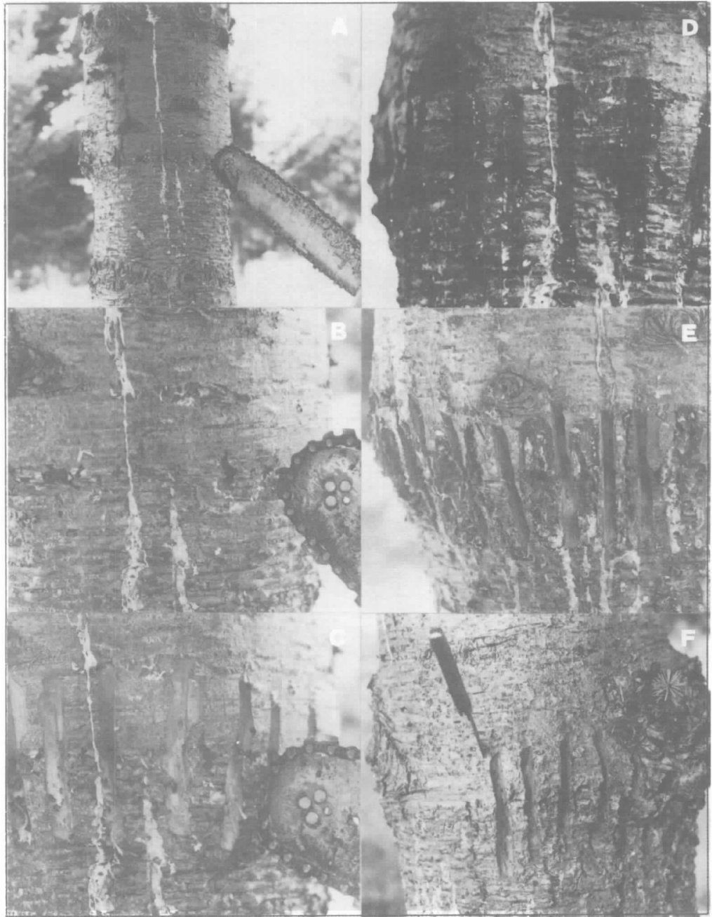
Figure 2—Method of bark scoring Douglas-fir graft unions with a small, gas-powered chain saw. (A) The defective graft union area. (B) Incipient bark decline is indicated by the presence of a line of pits or fissures along the union. (C) Newly cut bark scores in August 1983. (D) Healing of the 1983 cuts in August 1985. (E) Newly made bark scores of the second treatment in August 1985. The 1985 cuts were centered between the scars of the 1983 treatment. (F) Cuts were made only where brownline was found; the healthy areas of indeterminate unions (induced incompatibles) were not treated.
