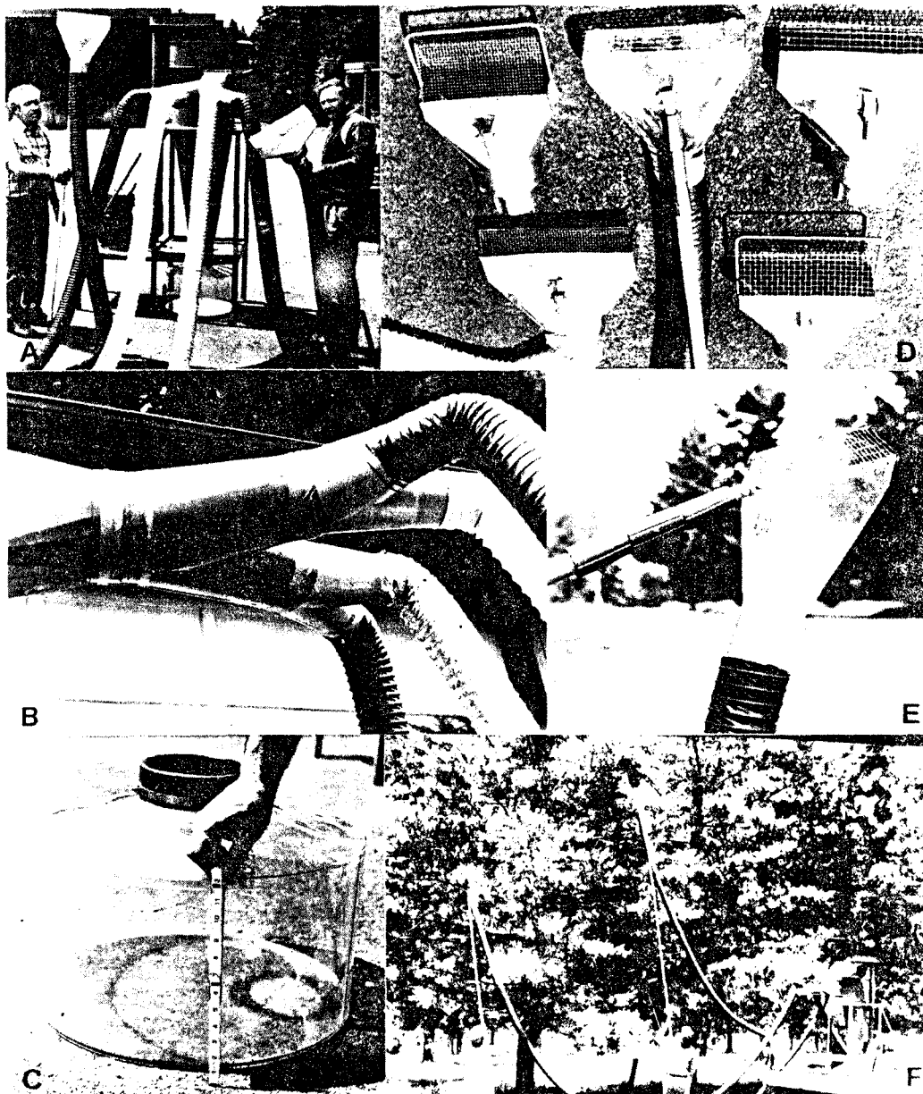
Figure 1—Cyclone dust collector and attachments. (A) Vacuum with collector and four mounted hoses. (B) Inlet manifold with 4-inch hoses attached. (C) Lexan collector drum with rubber connecting gasket. (D) Vacuum heads showing opening and width dimensions. (E) Lexan vacuum head attached to extension pole and hose. (F) Vacuuming pollen from sugar pine trees.
