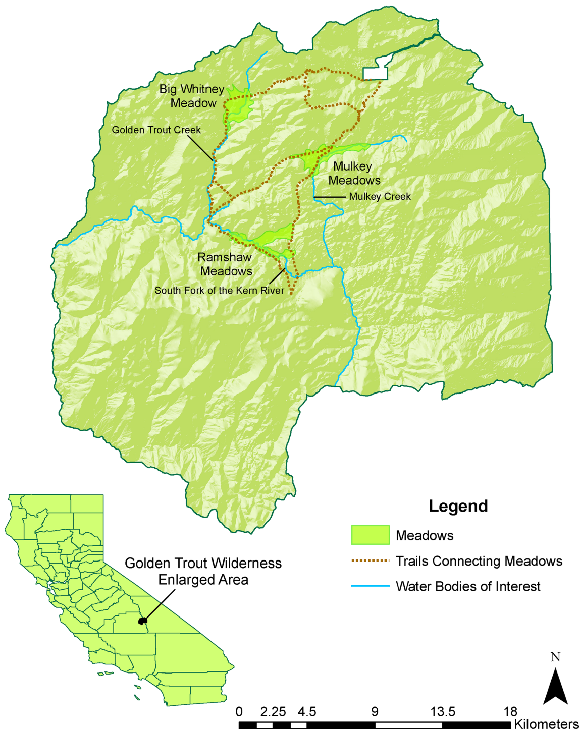
Fig 1. Study area. Data were collected in three distinct meadow systems of the Golden Trout Wilderness, California, a protected area within the Inyo National Forest in the Sierra Nevada mountains, which is the last remaining habitat of the Golden Trout ( Oncorhynchus mykiss aquabonita ). Water temperature was measured between 2008–2013 in three rivers: (1) Mulkey Creek, within Mulkey Meadows, between 2827–2844 m in elevation, (2) the South Fork of the Kern River within Ramshaw Meadows, between 2629–2648 m, and (3) the Golden Trout Creek within Big Whitney Meadow, between 2931–2964 m.
