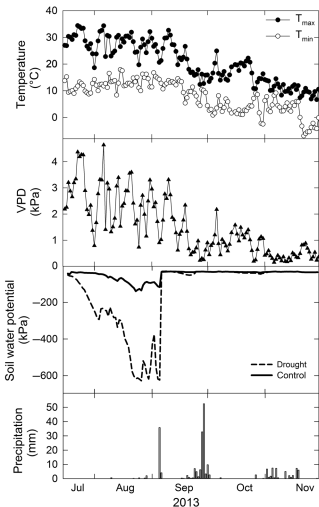
Figure 1. Maximum ( T_{\text{max}} ) and minimum ( T_{\text{min}} ) temperature, VPD, soil water potential and precipitation during the summer of 2013. Soil water potential was measured continuously at 10 cm. Large rain events in late summer effectively eliminated the drought treatment.
