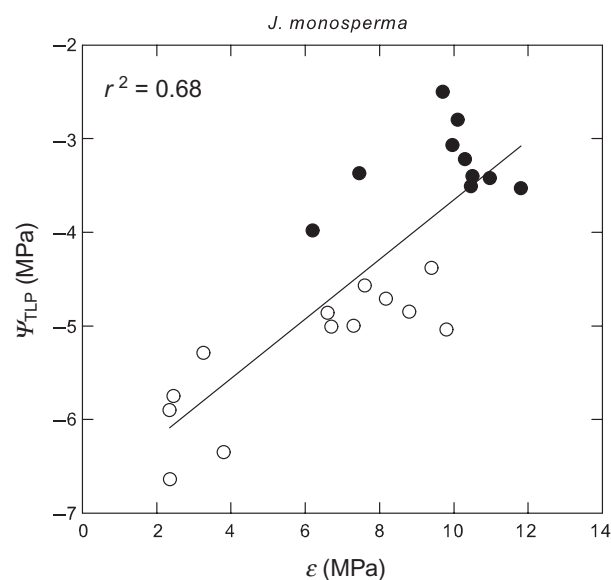
Figure 6. Relationship between the water potential at the turgor loss point ( \Psi_{TLP} ) and the bulk tissue modulus of elasticity ( \epsilon ) for (○) non-rehydrated and (●) rehydrated J. monosperma shoots excised on different dates during 2012–2013. Data taken from Fig. 3.
