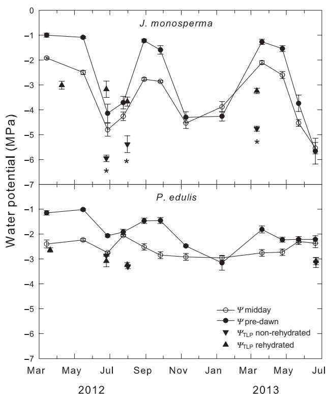
Figure 1. Seasonal courses of predawn and midday shoot water potential ( \Psi ) in co-occurring J. monosperma and P. edulis trees. Estimates of the shoot water potential at the turgor loss point ( \Psi_{TLP} ) obtained from pressure-volume curves for rehydrated and non-rehydrated shoots excised on different dates are shown. Asterisks indicate significant differences ( P \leq 0.01 ) in \Psi_{TLP} between rehydrated and non-rehydrated shoots.
