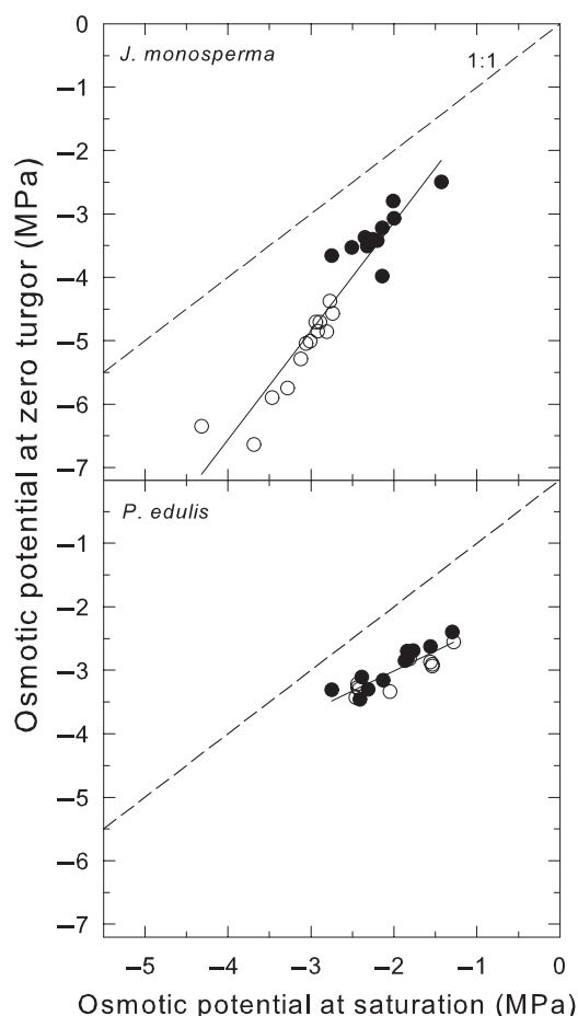
Figure 5. Relationships between the osmotic potential at zero turgor (turgor loss point) and the osmotic potential at saturation determined from pressure-volume curves for (●) rehydrated and (○) non-rehydrated shoots of J. monosperma and P. edulis . Regressions are significant at P < 0.0001 .
