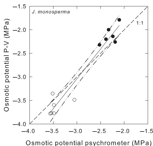
Figure 7. Relationship between osmotic potential determined from pressure-volume curves and osmotic potential measured in psychrometer chambers on frozen, thawed and crushed tissue samples from (●) rehydrated and (○) non-rehydrated shoots from six individuals of J. monosperma . The diagonal dashed line represents a 1:1 relationship and the dashed-dotted lines represent the 95% confidence interval for the solid regression line ( r^2 = 0.94 , P < 0.0001 ).
