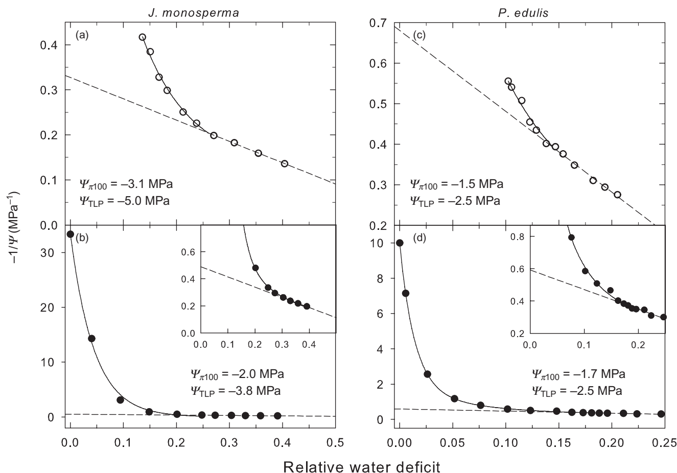
Figure 2. Representative pressure-volume curves for a non-rehydrated (a) and rehydrated (b) shoot collected from the same J. monosperma plant on 12 March 2013 and a non-rehydrated (c) and rehydrated (d) shoot collected from the same P. edulis plant on 24 June 2013. The shoot water potentials at the time of excision in a and c were -2.4 MPa and -1.8 MPa, and -0.03 and -0.1 MPa after rehydration in b and d. Note difference in x- and y-axis scales among the panels. Osmotic potentials at saturation ( \Psi_{\pi 100} ) and the water potential at the turgor loss point ( \Psi_{TLP} ) are shown. Insets in b and d show expanded axis scales for the region of the curve near turgor loss.
