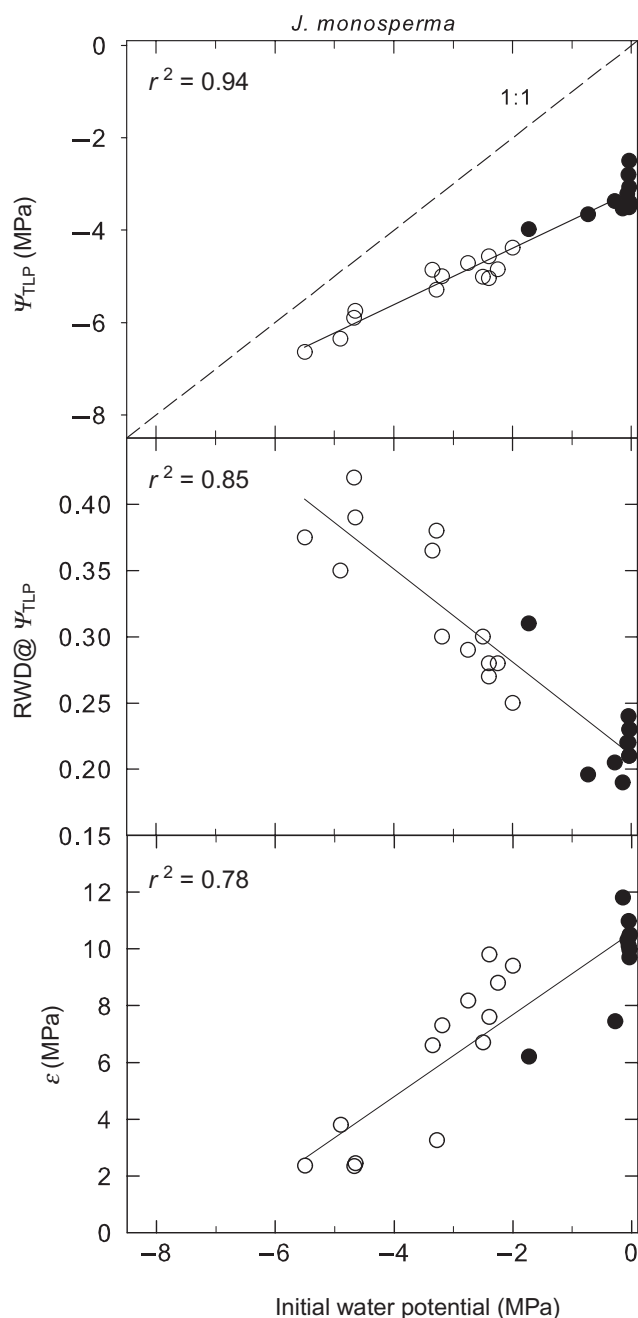
Figure 3. Relationships between initial shoot water potential and (a) the water potential at the turgor loss point ( \Psi_{\text{TLP}} ), (b) the relative water deficit at the turgor loss point ( \text{RWD}@ \Psi_{\text{TLP}} ), and (c) the bulk tissue modulus of elasticity ( \epsilon ) for (○) non-rehydrated and (●) rehydrated J. monosperma shoots excised on different dates during 2012–2013.
