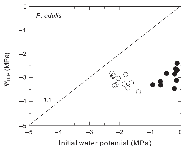
Figure 4. Relationship between the turgor loss point estimated from pressure-volume curves and the initial water potential for (●) rehydrated and (○) non-rehydrated shoots of P. edulis collected on different dates during 2012–2013.
