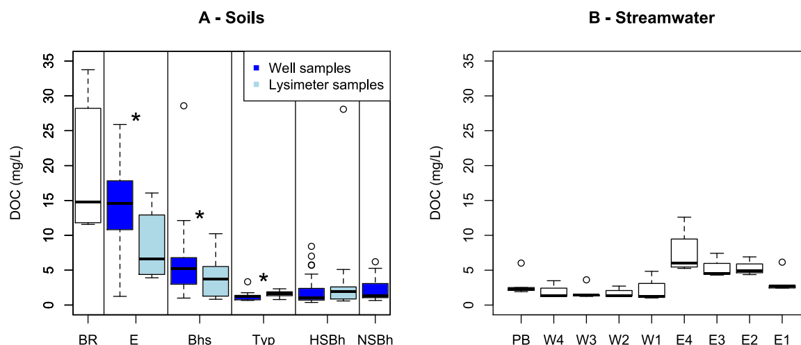
Figure 4. Concentration of DOC (mg/L) in bedrock runoff (BR) and groundwater, and lysimeter samples in (a) the five HPUs and at (b) the outlets of WS3 (Paradise Brook, PB) and eight tributaries in WS3. Figure 4a shows groundwater and lysimeter water for each HPU except near-stream Bh podzols (NSBh), as no lysimeter samples were available. For bedrock runoff (BR), n = 5 . For E podzols (E), n = 45 for groundwater and 12 for lysimeter samples. For Bhs podzols (Bhs), n = 66 for groundwater and 28 for lysimeter. For typical podzols (Typ), n = 17 for groundwater and 16 for soil water. For hillslope Bh podzols (HSBh), n = 77 for groundwater and 31 for lysimeter samples. Finally, for near-stream Bh podzols, n = 11 for groundwater. A star shown between two grouped soil water and groundwater boxplots indicates a significant difference according to a Wilcoxon rank sum test, p -value < 0.05 . Figure 4b shows DOC in stream water for all sample dates in Zimmer et al. [2013] at the outlet of WS3 (Paradise Brook, PB), four tributaries on the western side of the catchment (W1, W2, W3, and W4) and four tributaries on the eastern side of the catchment (E1, E2, E3, and E4). The middle line in each box corresponds to the median of the data, the hinges are the boundaries of the inter-quartile range (IQR), the whiskers are the first and third quartile \pm 1.5 times the IQR, and points are outliers beyond the range of the whiskers.
