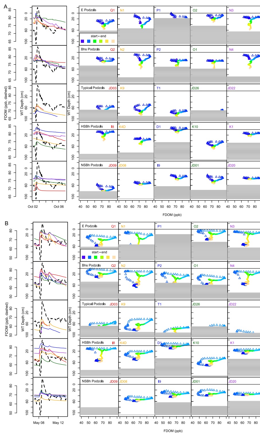
Figure 6. FDOM at the catchment outlet and water table at five example wells in each HPU. Figure 6a is an event occurring on 2 October 2011 and Figure 6b is from 7 May 2012. In the plots on the left, FDOM is indicated by a dashed line and water table levels are indicated by colored solid lines. The color of each well record on the left corresponds to the well name of the same color in the plots on the right. Plots on the right are water table (y axis) plotted against catchment outlet FDOM (x axis), the color of the plots goes from blue at start to beige at the end of the event. Points on the rising limb of the FDOM time series are shown as upward facing, open triangles and points on the falling limb are shown as smaller, filled diamonds. The filled grey area at the bottom of the plots on the right denotes the C horizon at each well. A horizontal line at the ground surface (0 depth) is shown for each plot on the right.
