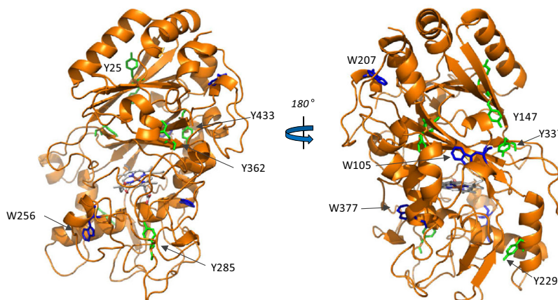
Fig. 3. Location of four tryptophan (blue sticks) and seven tyrosine (green sticks) residues on ribbon representation of the recombinant AauDyP crystal structure (PDB 4W7J) from two different orientations (180° rotation). The heme cofactor is also shown as CPK-colored sticks. See Fig. 2A for helix and \beta -strand identification.
