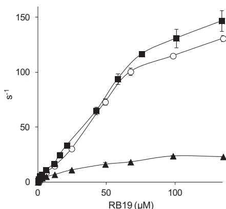
Fig. 5. Kinetics of Reactive Blue 19 oxidation by native AauDyP (circles) and its Y337S (squares) and W377S (triangles) variants. Reactions were performed using 10 nm enzyme, 0.1 mM H_2O_2 and different RB19 concentrations. Means and 95% confidence limits are shown. Adapted from Linde et al. [20].
