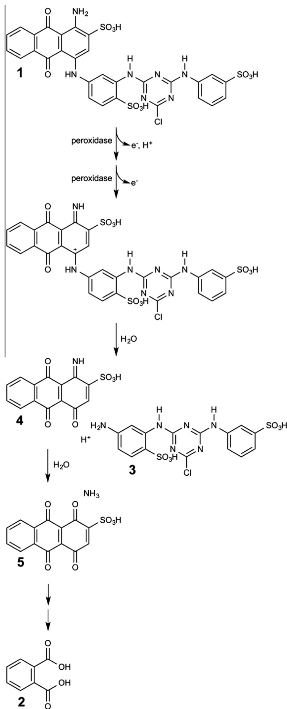
Fig. 6. Abbreviated pathway for the oxidation of Reactive Blue 5 (structure 1 ) by a conventional peroxidase mechanism, followed by spontaneous cleavage of the anthracenetetrone (structure 5 ) released. See the corresponding text for identity of the different intermediate compounds.
