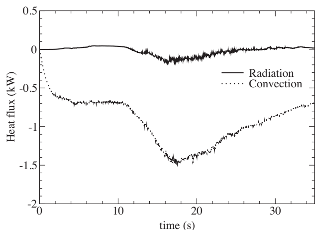
Fig. 16. Time history of global radiation and convection fluxes for a case with FMC of 80%. Positive heat flux means heat is transferred from gas to solid particle and negative heat flux means vice versa.
