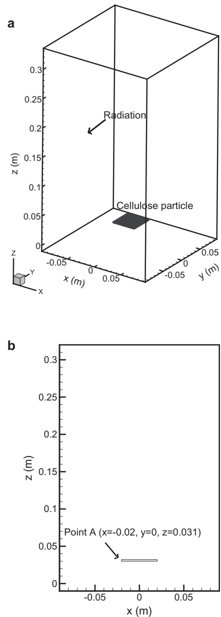
Fig. 2. (a) Isometric view of computational domain showing thin cellulose particle subjected to radiative heating from surface at x = -0.09 m and (b) two-dimensional view of computational domain along the xz -slice at y = 0 . Point A located at x = -0.02 m, y = 0 , z = 0.031 m is considered for analysis.
