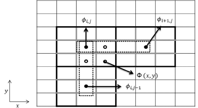
Fig. 1. Schematic representing bilinear interpolation used to couple the solid fuel domain solver variables to gas-phase solver variables; top view of xy -slice at the interface of solid fuel and gas-phase domain.
