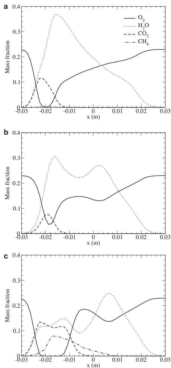
Fig. 12. Variation of mass fraction of tracked gas species at time (a) 5 s (b) 7.5 s and (c) 11 s along x at y = 0 and z = 0.035 m in the gas phase domain for a case with an initial FMC of 80%.
