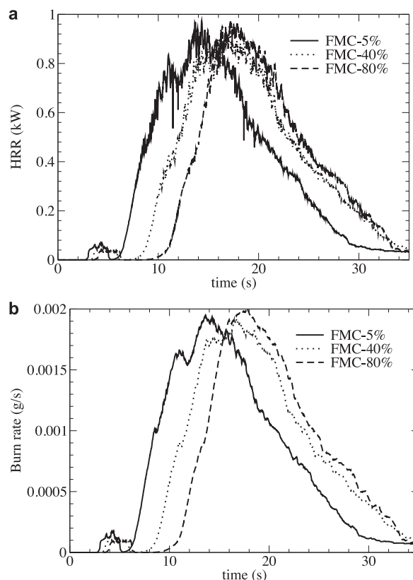
Fig. 8. Time history of (a) heat release rate and (b) burn rate in the gas phase for three cases with an initial FMC of 5%, 40% and 80%.
