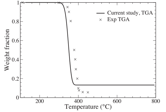
Fig. 4. Verification of results of current study using Gpyro TGA setup (solid line) with experimental TGA data [68] (crossmarks).
