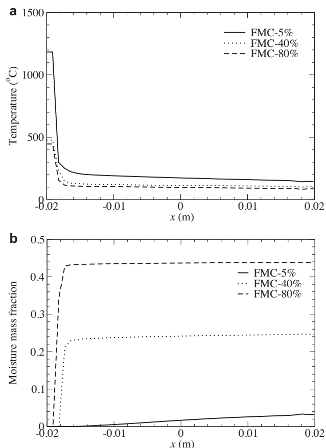
Fig. 6. Variation of (a) temperature and (b) mass fraction of moisture along x at y = 0 and z = 0.031 m at time 5 s in the solid phase for three cases with an initial FMC of 5%, 40% and 80%.
