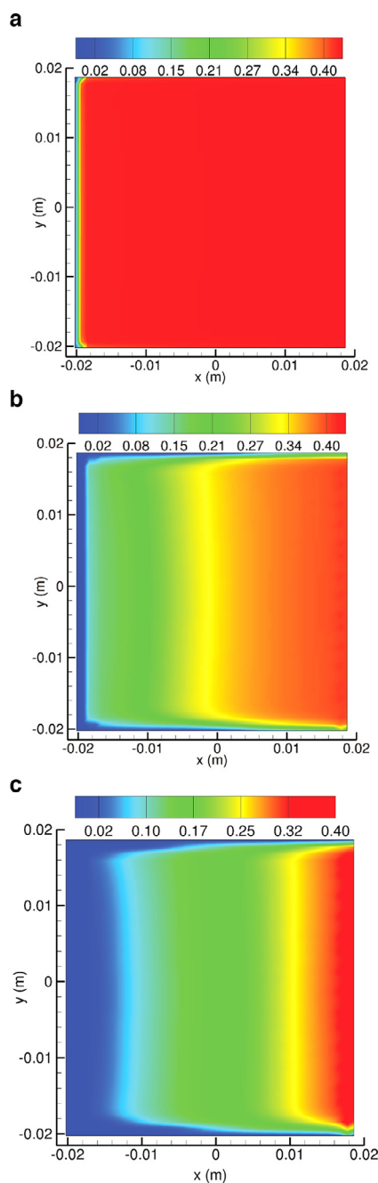
Fig. 11. Contours of moisture mass fraction in the solid fuel along x at (a) t = 5 s (b) t = 6.5 s and (c) t = 7.75 s on an xy -slice located at z = 0.031 m for a case with an initial FMC of 80%.
