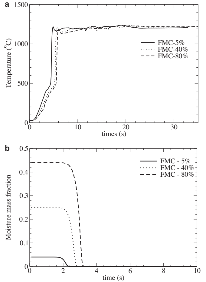
Fig. 5. Time history of (a) temperature, and (b) mass fraction of moisture at point A (see Fig. 2) for three cases with an initial FMC of 5%, 40% and 80%.
