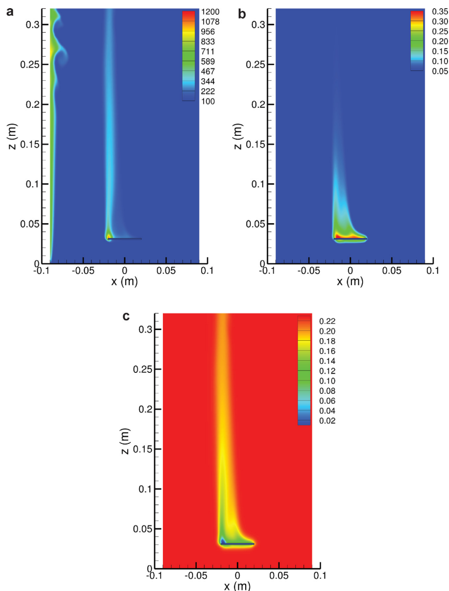
Fig. 14. Gas phase contours of (a) temperature (°C), (b) water vapor mass fraction and (c) oxygen mass fraction along x at t = 7.5 s on an xz -slice located at y = 0 for a case with an initial FMC of 80%.
