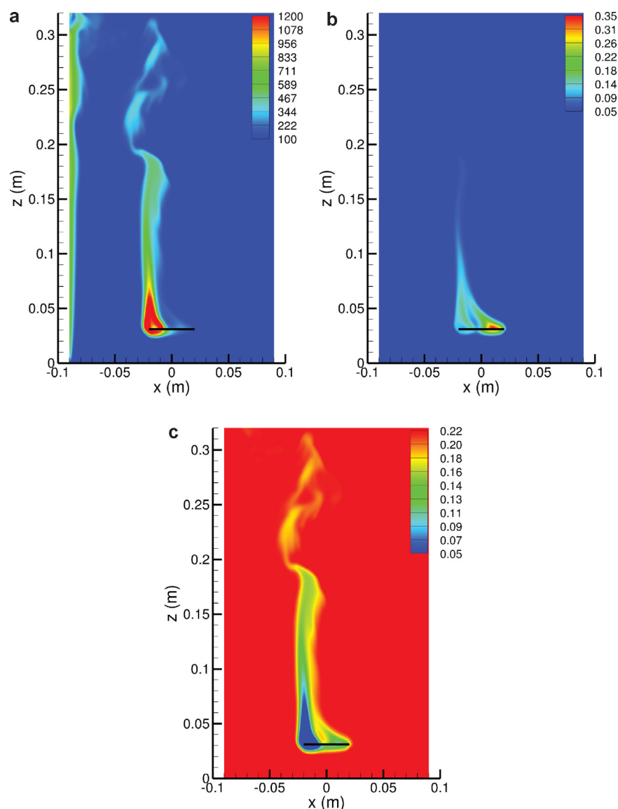
Fig. 15. Gas phase contours of (a) temperature (°C), (b) water vapor mass fraction and (c) oxygen mass fraction along x at t = 11 s on an xz -slice located at y = 0 for a case with an initial FMC of 80%.
