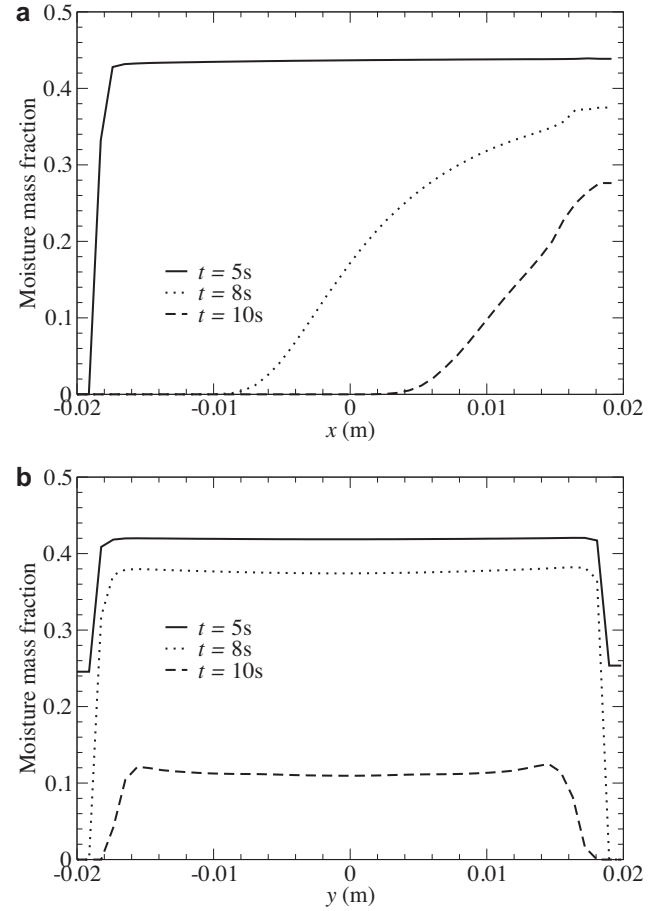
Fig. 10. Variation of moisture mass fraction (a) along x at y = 0 and z = 0.031 m and (b) along y at x = 0.0125 m and z = 0.031 m at various times in the solid phase for a case with an initial FMC of 80%.
