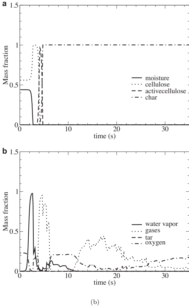
Fig. 9. Time history of (a) solid species and (b) gas species in the solid phase for a case with an initial FMC of 80% at point A.
