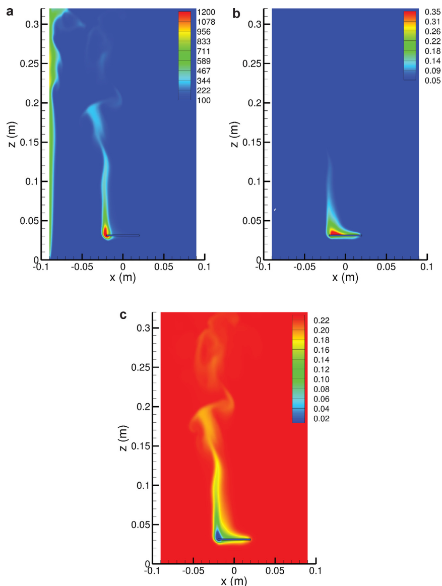
Fig. 13. Gas phase contours of (a) temperature (°C), (b) water vapor mass fraction and (c) oxygen mass fraction at t = 5 s on an xz-slice located at y = 0 for a case with an initial FMC of 80%.
