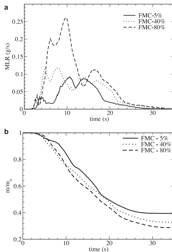
Fig. 7. Time history of (a) mass loss rate and (b) normalized mass in the solid phase for three cases with an initial FMC of 5%, 40% and 80%.
