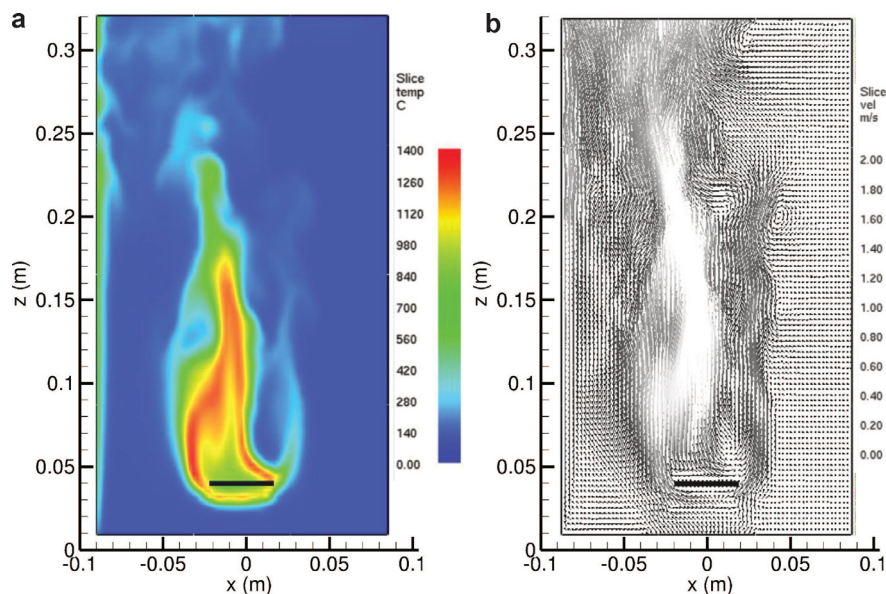
Fig. 17. (a) Gas phase temperature contours ( ^{\circ}C ), and (b) velocity vectors at time 15 s on an xz -slice located at y = 0 for a case with an initial FMC of 80%.
