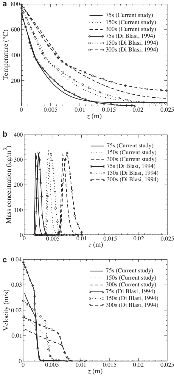
Fig. 3. Verification of results of current study using Gpyro for cellulose pyrolysis with simulations of Blasi [28] along the length of the specimen at different times; (a) temperature, (b) mass concentration of active cellulose and (c) velocity of gas species.
