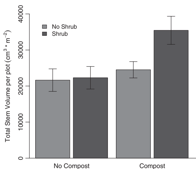
Figure 3. Treatment effects per plot for total stem volume. The effects of the interaction between the shrub and compost treatment are clearly apparent, with composted plots containing shrubs having significantly more stem volume compared with the other treatments. Error bars represent \pm SE. The number of replicates are as follows: no shrub/no compost, n = 14 ; no shrub/compost, n = 13 ; shrub/no compost, n = 14 ; shrub/compost, n = 13 . See Table 2 for treatment coefficients and p values.
