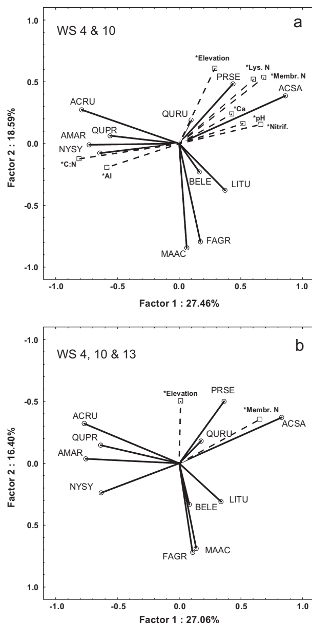
Fig. 5. Principal component analysis of tree species with a relative importance (dominance + density + frequency) \geq 5\% in WS 4, 10, or 13 at the FEF. Supplementary variables projected onto the factor space are: Elevation; Membr. N = \text{NO}_3 captured by anion resin membranes; Lys. N = lysimeter \text{NO}_3 concentrations; Nitrif. = potential net nitrification; pH = soil pH in water; Ca = exchangeable Ca; Al = exchangeable Al; and C:N = soil carbon-to-nitrogen ratio. Species codes are the same as those used in Fig. 3.
