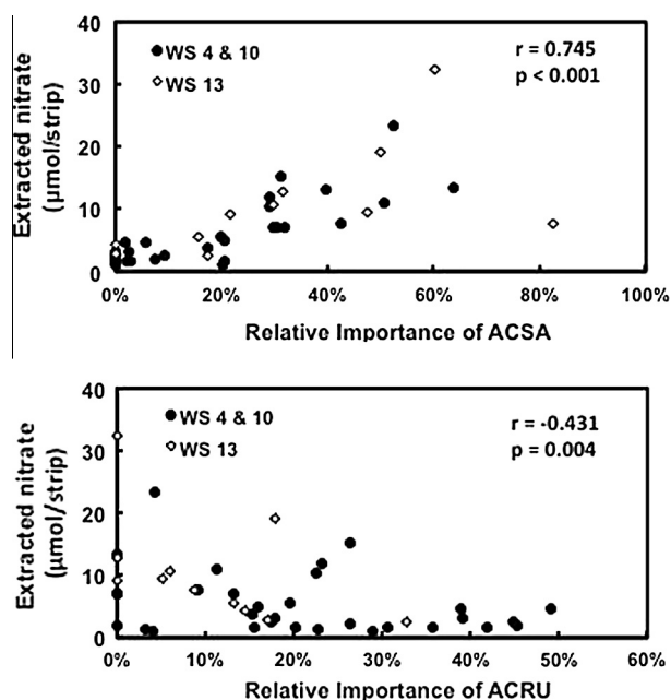
Fig. 4. The strongest positive and negative correlations found in small plots between \text{NO}_3 availability (assessed with anion resin membranes) and the relative importance (dominance + density) of individual tree species. Species codes are: ACSA = Acer saccharum , and ACRU = Acer rubrum .
