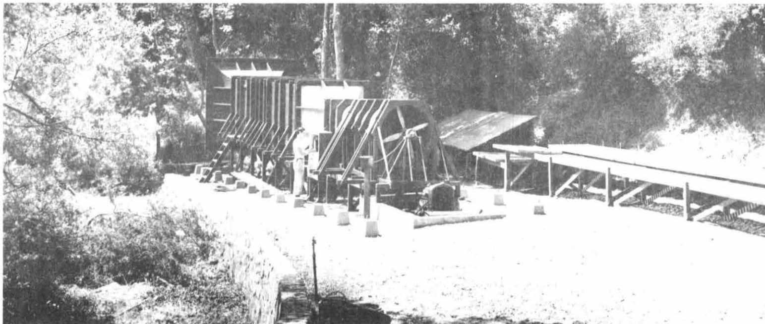
Figure 11.--Eiffel type low velocity wind tunnel used in the experiments.
