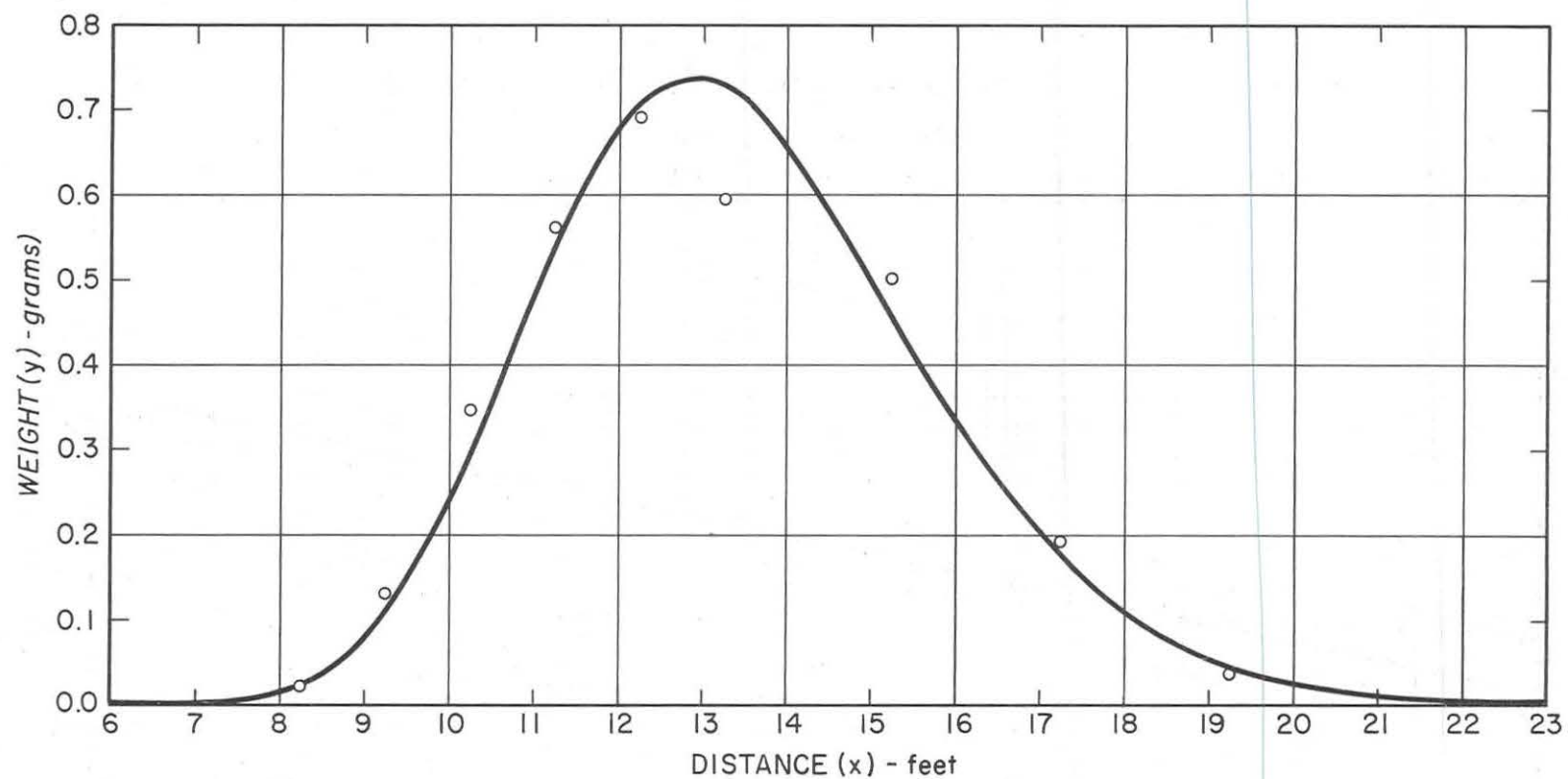
Figure 15.--Comparison of computed curve with experimental data.
