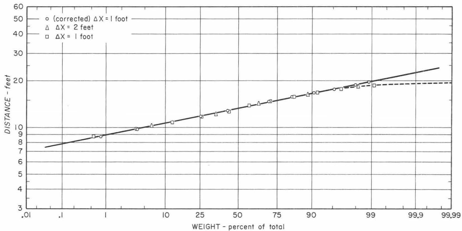
Figure 14.--Analysis of experimental run No. 108.
