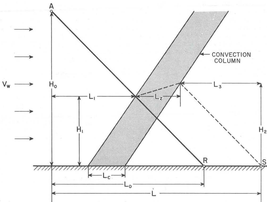
Figure 1.--Fall of a single particle through an idealized convection column.
