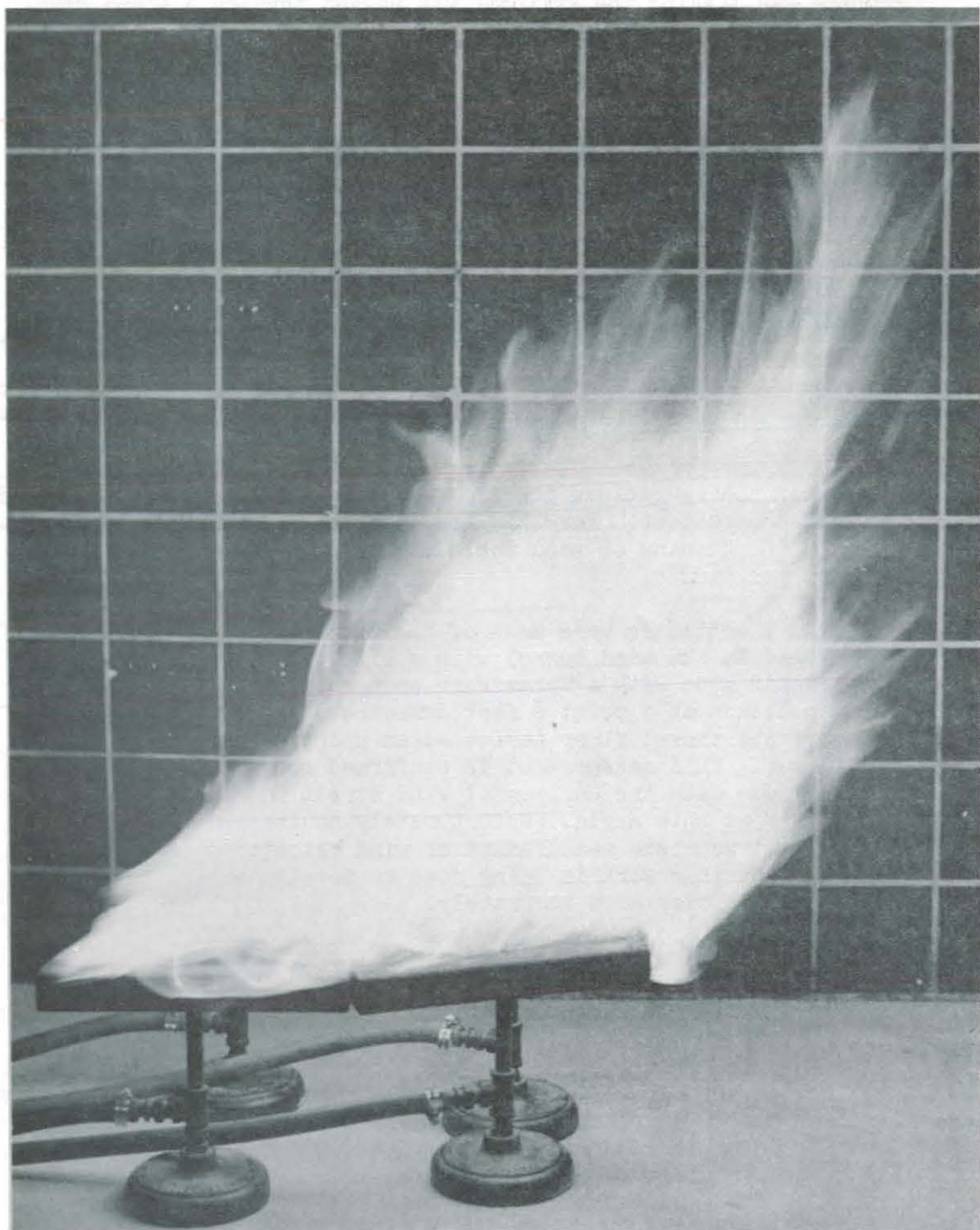
Figure 10.--"V" configuration of gas burners.
