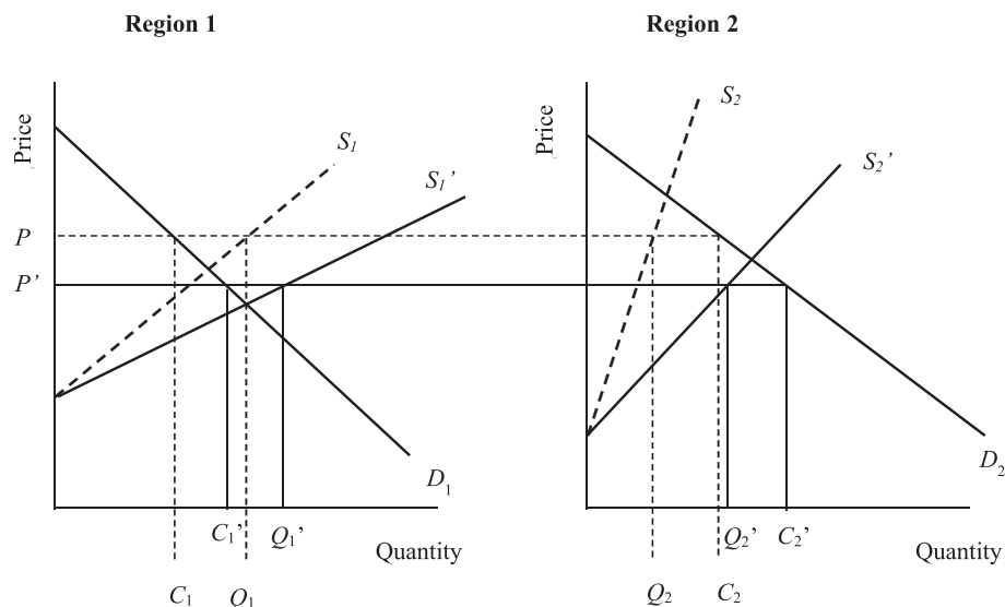
Fig. 1 Theoretical effects of supply shifts induced by CO 2 fertilization of forest stock on the production, consumption, trade, and price of wood in two trading regions. Dotted lines refer to the situation without CO 2 fertilization and the solid lines with CO 2 fertilization
