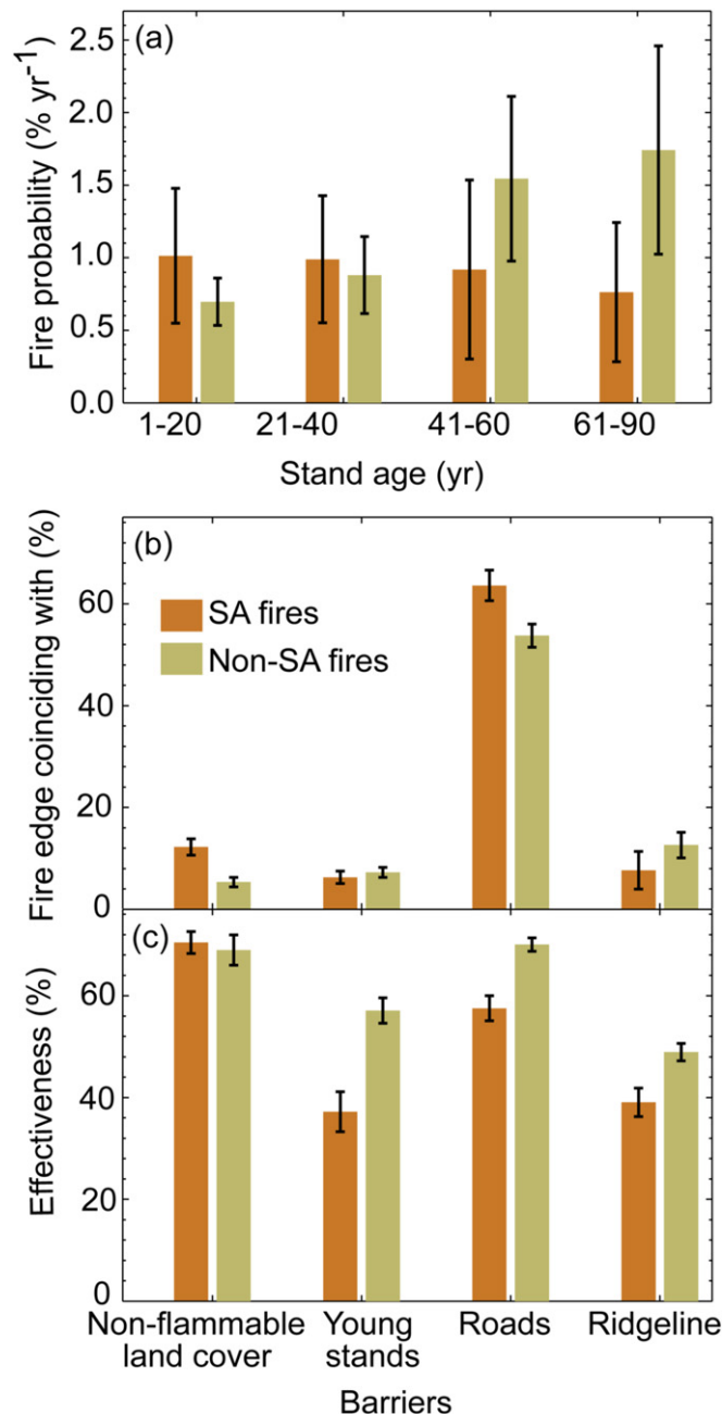
Figure 3. Effects of stand age and fuel breaks on fire probability. In panel (a), fire probability was calculated as the percent of area burned for each age group over the total available vegetated land area for the same age group in each year during 1959–2009. Panel (b) shows the percentage of fire perimeter length affected by non-flammable land cover types, stands 20 years or younger, roads, and ridgelines. Non-flammable land cover types included urban, agriculture, and ocean/lake, and additionally deserts and high elevation barren areas for non-SA fires. The effectiveness of a potential barrier (c) was calculated as the percentage of its presence in the 1 km buffered area outside of the fire perimeter over the total within fire-affected and buffered areas.
