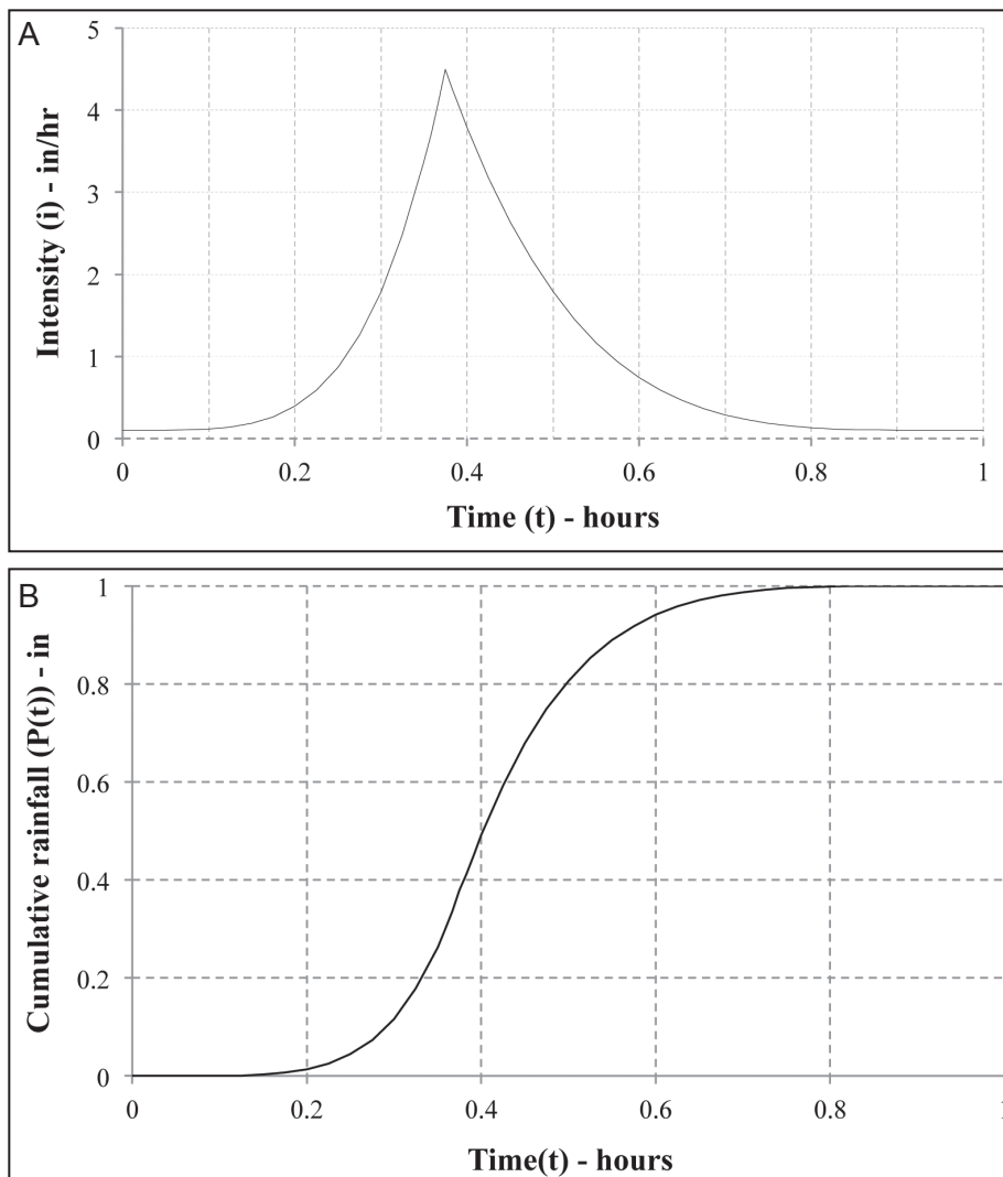
Figure 3-01 —Definition figures, for the case of P = 1 in, T = 1 hr, t_p = 0.375 hr, i_o = 0.20 in/hr, and i_p = 4.5 in/hr. For these conditions, n = 4.3 . Note that the intensity (A) shows on the cumulative rainfall (B) as the slope of the curve. The maximum slope occurs under the peak at 0.375 hr. This rainfall distribution is similar to the NEH4B distribution.
