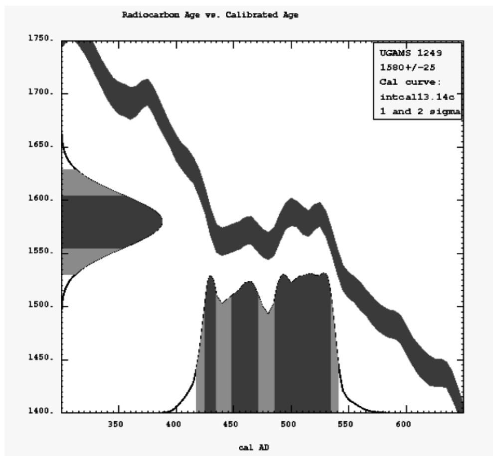
Figure 2—A calibration graph for converting radiocarbon date (Y-axis) to calendar date (X-axis).
