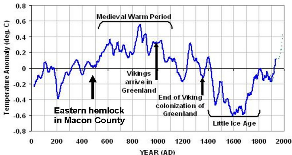
Figure 6—A global temperature reconstruction based on non-tree ring proxies (Loehle and McCulloch 2008). Data for this graph is online at www.econ.ohio-state.edu/jhm/agw/loehle/ . Hemlock was growing in Macon County, Alabama prior to the Medieval Warm period.
