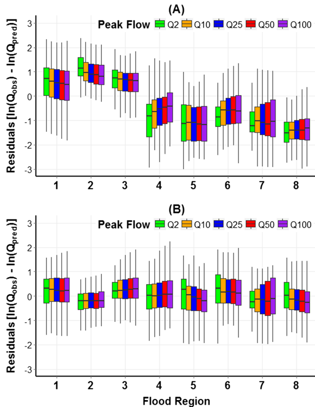
Figure 6. Average residuals across all peak flows ( Q , \text{m}^3/\text{s} ) and flood regions using (A) drainage area alone as a predictor of peak flows and (B) five principal components along with drainage area as predictors of peak flows. The line inside the box represents the median value, the box itself represents the interquartile range IQR (25th–75th percentile range) and the whiskers are the lowest and highest values that are within 1.5 \times \text{IQR} of the 25th and 75th percentiles
