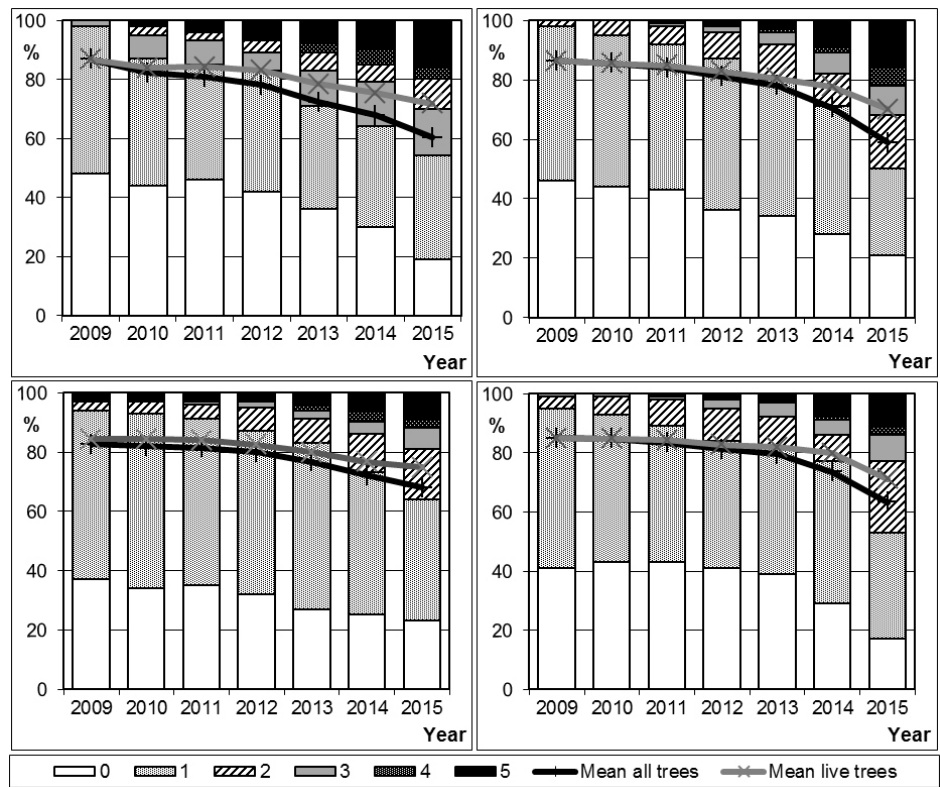
Figure 2: Trends in the mean annual foliage of all (black line) and live ash trees (grey line) and degrees of defoliation (1-5) in the mixed forest stand on permanent research plots
