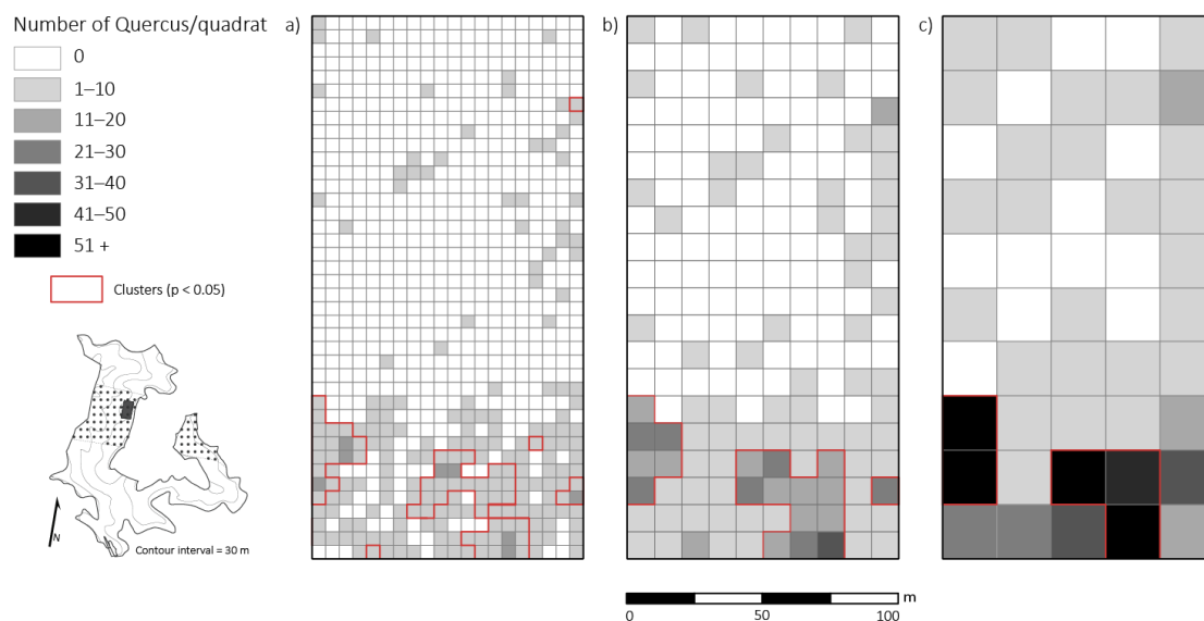
Figure 5. Distribution of small-sized Quercus stems across a 2 ha plot four years after canopy disturbance in a Quercus dominated stand within the Sipsey Wilderness, Alabama, USA. The red outlines represent the significant clustering ( p < 0.05 ) of small-sized Quercus stems. Inset map shows the Quercus stand boundary, tornado swath (dotted pattern), plot location, and topography. (a) 5 \times 5 m; (b) 10 \times 10 m; (c) 20 \times 20 m. See Figure 1 for disturbance class delineations.
