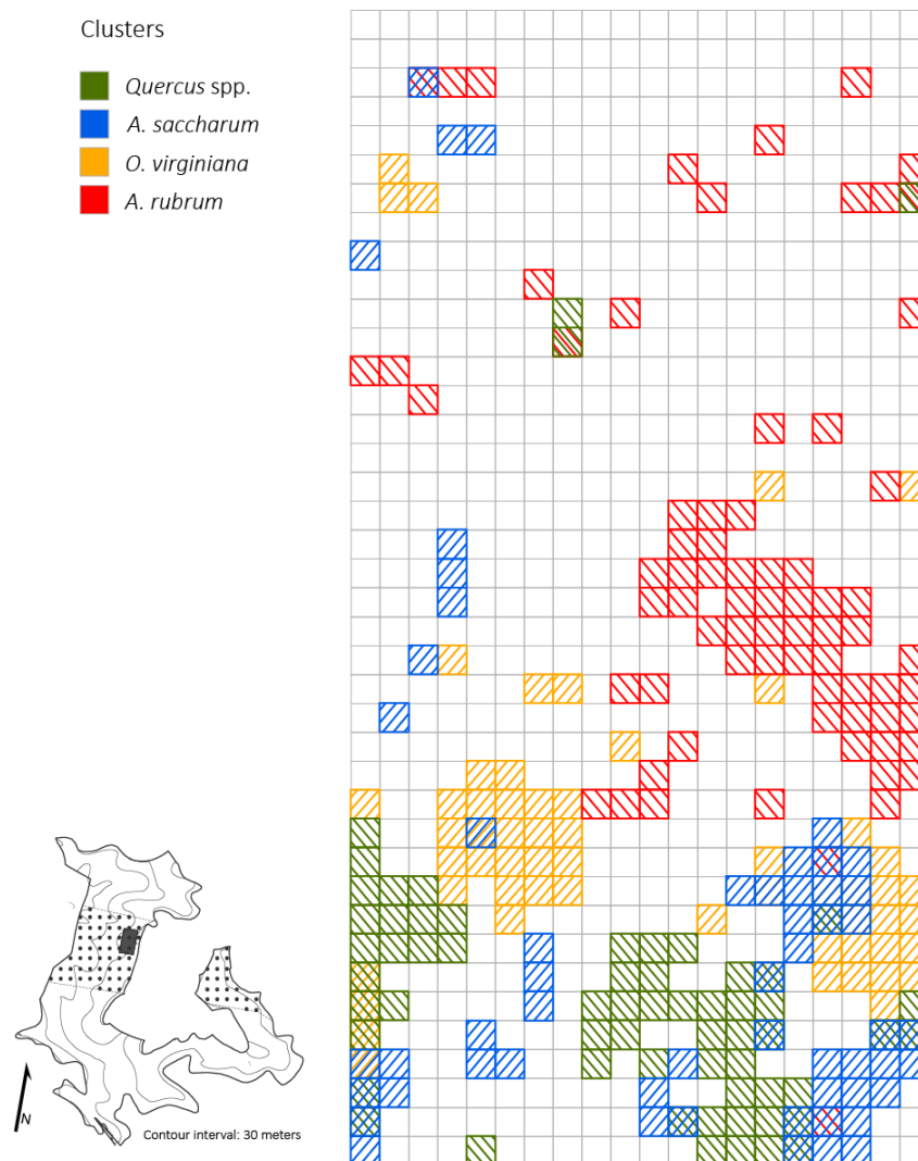
Figure 6. Distributions of Quercus spp., A. saccharum , O. virginiana , and A. rubrum clusters across a 2 ha plot ( 5 \times 5 m resolution) four years after canopy disturbance in a Quercus dominated stand within the Sipsey Wilderness, Alabama, USA. Inset map shows the Quercus stand boundary, tornado swath (dotted pattern), plot location, and topography. See Figure 1 for disturbance class delineations.
