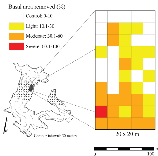
Figure 1. Spatial distribution of disturbance classes in a 2 ha plot based on estimated basal area removed by a wind event in a Quercus dominated stand within the Sipsey Wilderness, Alabama, USA. Inset map shows the Quercus stand boundary, tornado swath (dotted pattern), plot location, and topography.
