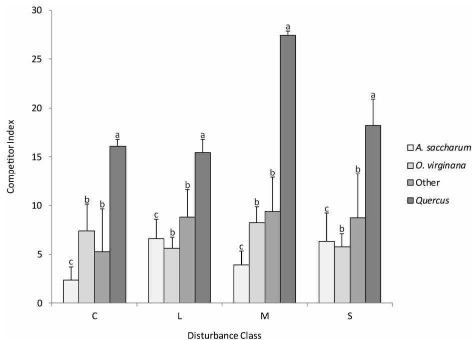
Figure 2. Average competitor indices with standard errors for competitor species (0.5–5.5 m height) by taxonomic group in the control neighborhood (C), and light (L), moderate (M) and severe (S) disturbance class neighborhoods. Bars with different lowercase letters within taxonomic groups represent significant differences ( p < 0.05 ) among species competitive ability. CI did not vary significantly ( p < 0.05 ) by disturbance classes.
