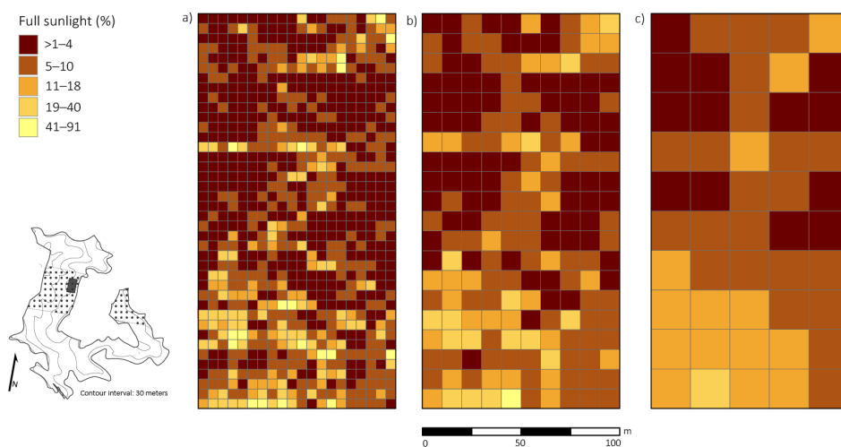
Figure 3. Spatial distribution of percent full sunlight taken at 1.47 m above the ground across a 2 ha plot four years after canopy disturbance in a Quercus dominated stand within the Sipsey Wilderness, Alabama, USA. Inset map shows the Quercus stand boundary, tornado swath (dotted pattern), plot location, and topography. (a) 5 × 5 m; (b) 10 × 10 m; (c) 20 × 20 m. See Figure 1 for disturbance class delineations.
