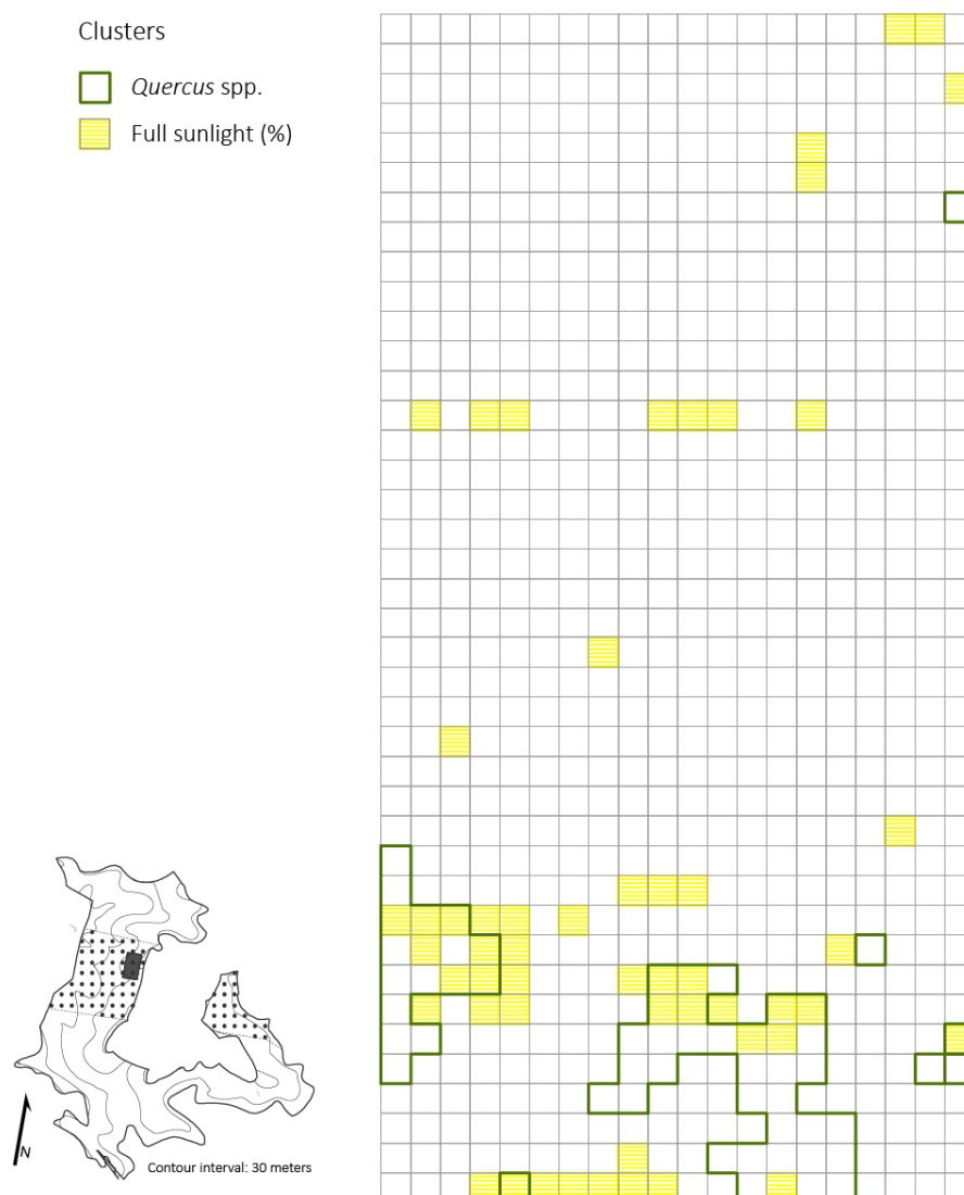
Figure 4. Distributions of Quercus spp. clusters and high light clusters based on percent of full sunlight across the 2 ha plot ( 5 \times 5 m resolution) four years after the disturbance in a Quercus dominated stand within the Sipsey Wilderness, Alabama. Inset map shows the Quercus stand boundary, tornado swath (dotted pattern), plot location, and topography. See Figure 1 for disturbance class delineations.
