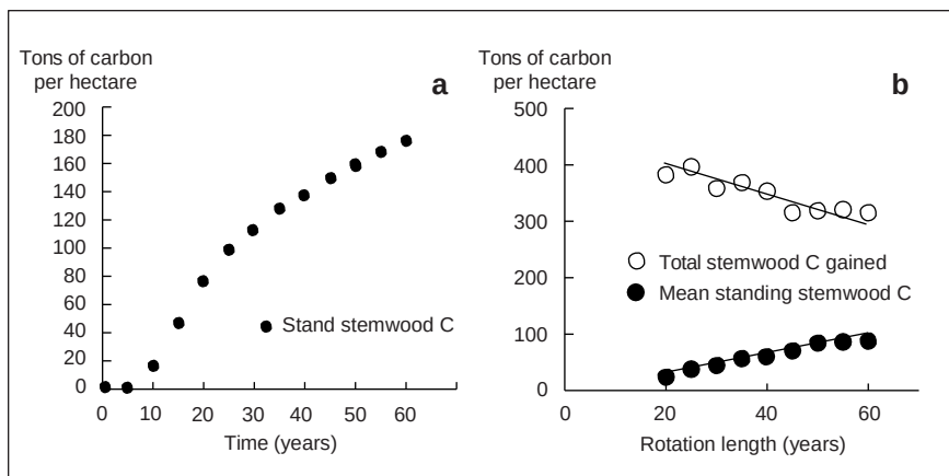
Figure 4. (a) Modeled carbon accretion (stemwood only) over time for an upper Coastal Plain loblolly pine stand with a site index of 80, and (b) total carbon gained and mean standing carbon as a function of rotation length, both calculated over a 100-year period.
