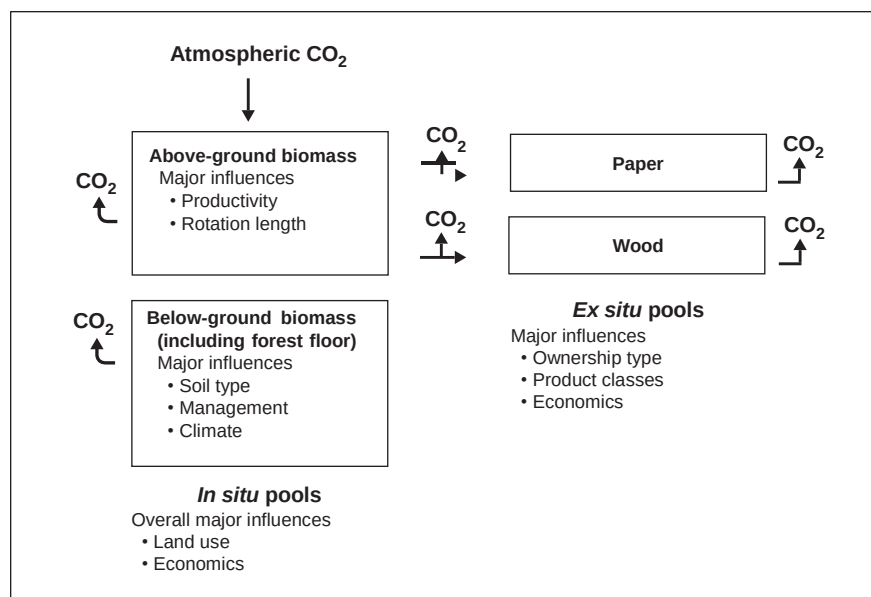
Figure 1. Conceptual model of carbon sequestration via southern pine forestry.
