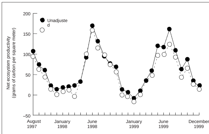
Figure 2. Monthly sums of net ecosystem carbon productivity (NEP) over a loblolly pine plantation at the Duke Forest. Positive NEP values represent uptake by the forest, whereas negative values indicate that release from decomposition and plant respiration is greater than net photosynthesis. Adjusted values represent estimates corrected for ecosystem respiration under stable nighttime conditions. Note that the drought during June 1999 drastically reduced carbon uptake relative to the previous June.
