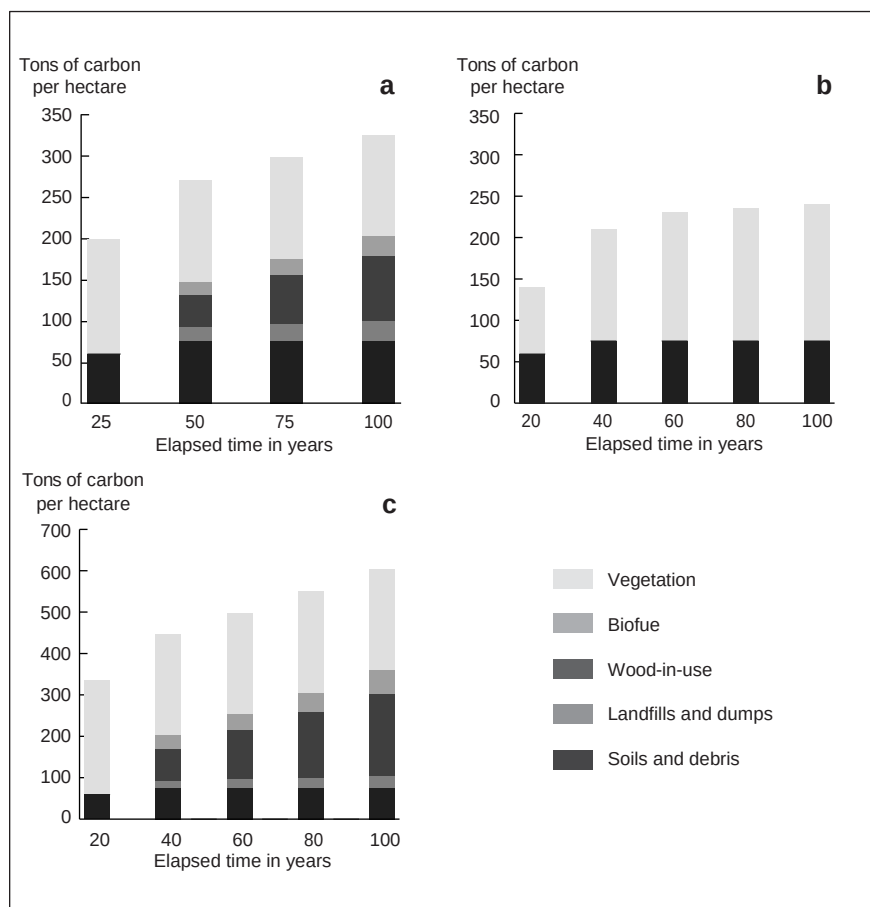
Figure 5. Integrated analysis of carbon sequestration using the model HARVCARB (from Row and Phelps 1996): (a) stand with site index of 75 and a 25-year rotation length; (b) an uncultivated, unharvested stand; and (c) stand managed to decrease rotation length to 20 years.
