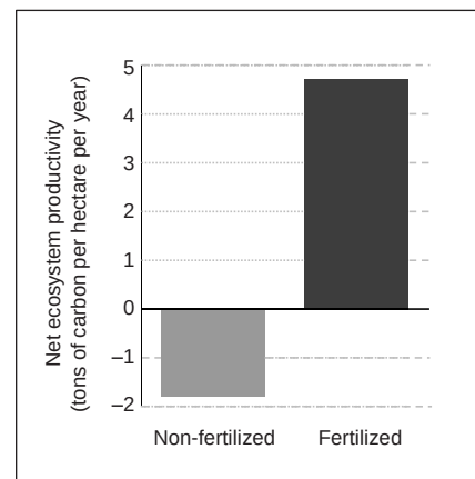
Figure 3. Net ecosystem productivity developed from component analysis for nonfertilized and fertilized 11-year-old loblolly pine plantations growing at the Southeast Tree Research and Education Site (SETRES), Laurinburg, North Carolina. The results are for the 1995 growing season, after four years of fertilization treatment. Source: Maier and Kress (2000).
