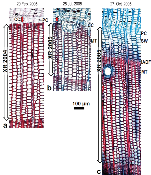
Figure 6. Wood formation in Pinus halepensis at Guardamar (GUA): a) The cambial cells (CC, red arrows) and post-cambial cells (PC) formed in 2005 to the outside of the 2004 growth ring (XR2004); b) Mature tracheids (MT) with no PC in the 2005 growth ring (XR2005); c) PC and cells with secondary wall thickening (SW) produced to the outside of the latewood MT and the intra-annual density fluctuation (IADF) (modified from De Luis et al. 2011a).
