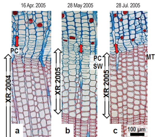
Figure 5. Wood formation in Pinus halepensis at Jarafuel (JAR): a) Cambium (red arrows) and post-cambial cells (PC) produced in 2005 to the outside of latewood of the 2004 growth ring (XR 2004); b) PC and cells with secondary wall thickening (SW) in the developing 2005 growth ring (XR 2005); c) Mature tracheids (MT) in the developing XR 2005.
