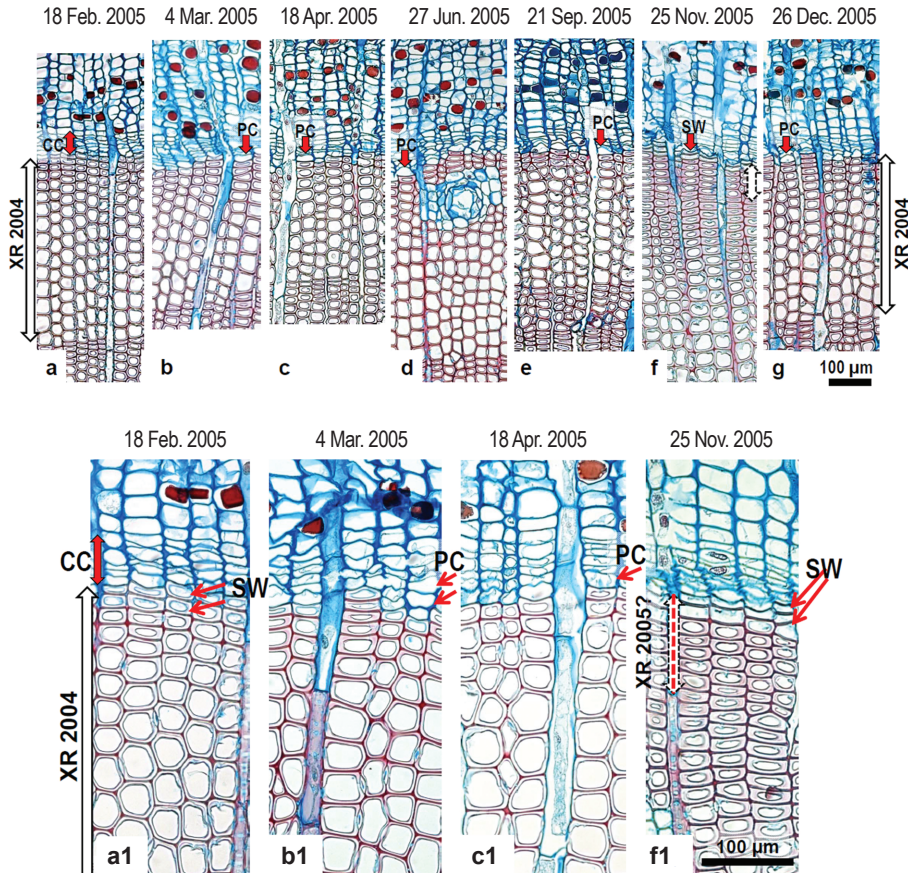
Figure 4. Time-course of cambial structure in a representative Pinus halepensis at Maigmo (MAI) (bark at top of section): (a–g) Cambial cells (CC), post-cambial derivatives (PC), and cells undergoing thickening of the secondary wall (SW) are marked. Mature xylem under CC was formed as part of the 2004 growth ring (XR 2004). (a1, b1, c1, f1) Detailed views of (a, b, c, and f). (a1) cells from 2004 completing secondary wall thickening in 2005 (SW); (b1, c1) PC cells (arrows); (f1) 2005 SW and latewood potentially formed in 2005 (XR 2005?) in the absence of 2005 earlywood.
