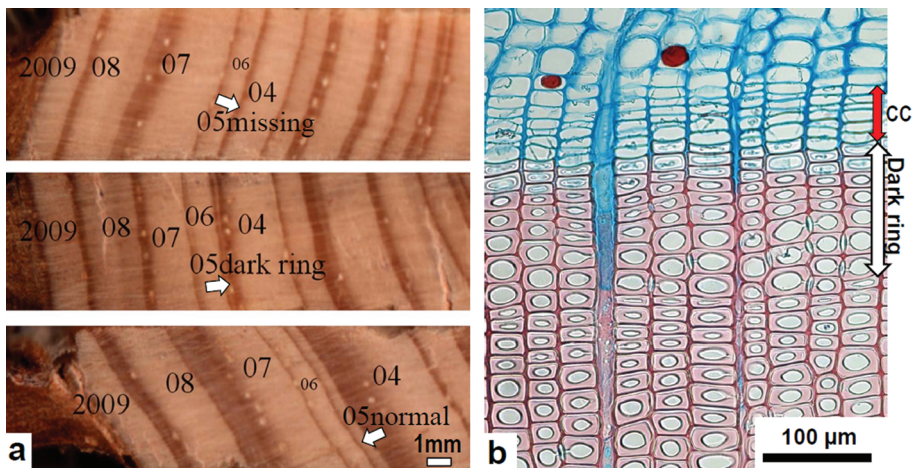
Figure 7. Pinus halepensis from MAI: a) Increment cores collected in 2009 (bark left) to show the 2005 (05) ring as missing (top), as a dark ring (middle), and normal (bottom); b) Stained cross section of sample collected in 2005 with the dark ring of latewood beneath the cambium (CC).
