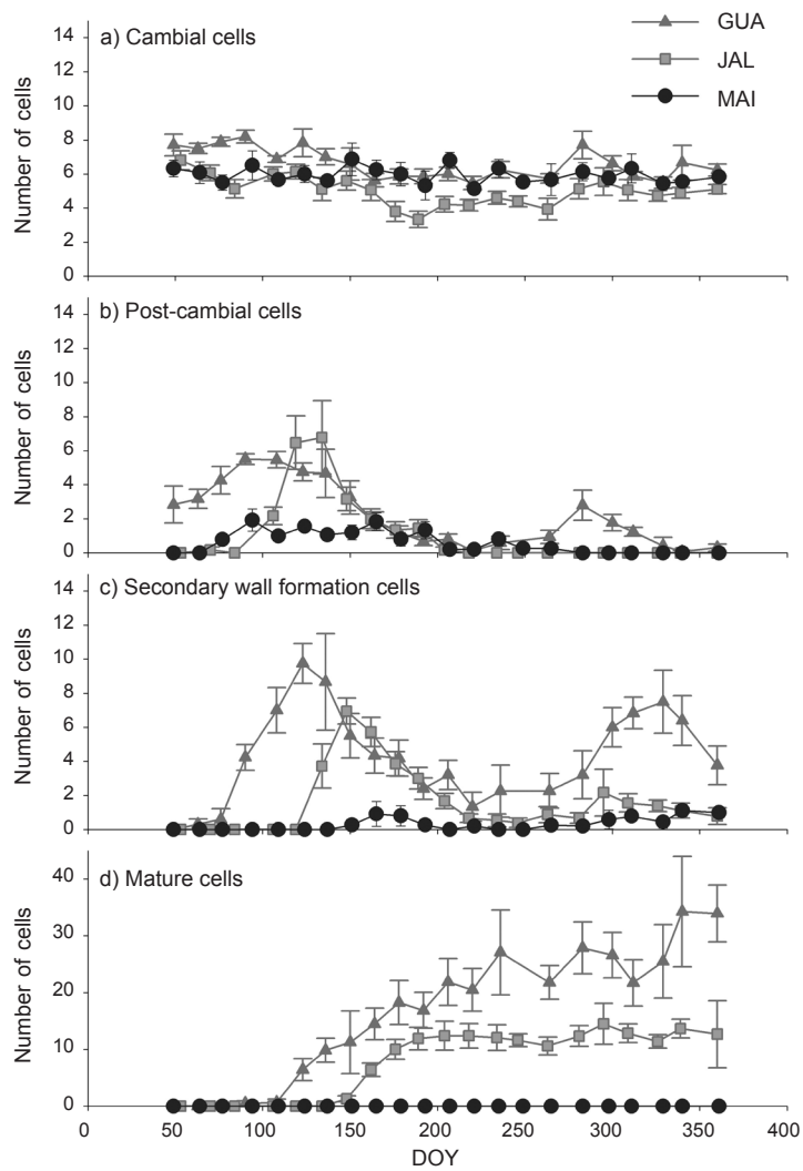
Figure 3. Wood formation dynamics at Maigmo (MAI), Guardamar (GUA), and Jarafuel (JAL) in 2005: a) average numbers and standard deviations of cambial cells (CC) per radial file, b) xylem cells in post-cambial growth (PC), c) tracheids undergoing secondary wall thickening and lignification (SW), and d) mature tracheids (MT).
