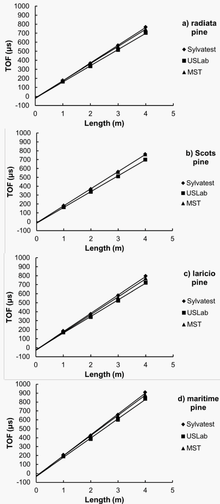
Fig. 6. Linear relationships between TOF and timber length (a-radiata pine; b-Scots pine; c-lario pine; and d-maritime pine)
