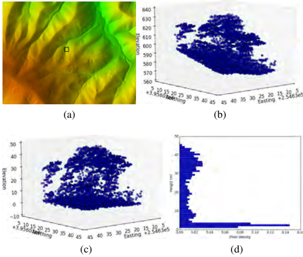
Fig. 3. (a) 3-D LiDAR point cloud at 30 m \times 30 m region (black square) in a typical GSMNP cove forest. (b) The raw LiDAR point cloud (3,985 points), showing the imprints of the underlying cove topography. (c) LiDAR point cloud after topographic detrending and filtering (3,936 points) that converted the elevations to above ground level elevation. (d) Distribution of LiDAR point density along the vertical profiles in a cove forest dominated by tall trees and a dense understory.
