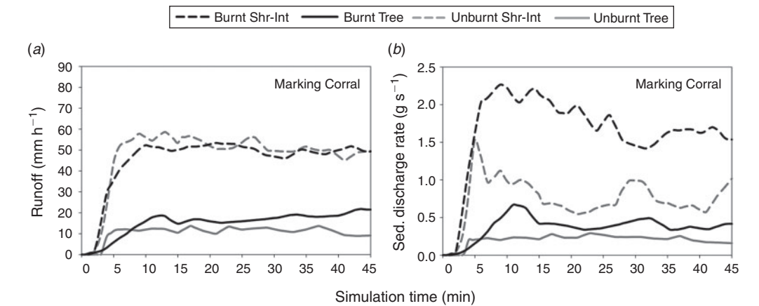
Fig. 2. Runoff hydrographs (a) and sedigraphs (b) for large-plot (13 m 2 ) rainfall simulations (102 mm h -1 , 45 min) that generated runoff on burnt (1 year post-fire) and unburnt (1 year pre-fire) tree (Tree; Pinus monophylla Torr. and Frém. or Juniperus osteosperma [Torr.] Little) and shrub–interspace (Shr-Int) zones at the Marking Corral study site.
