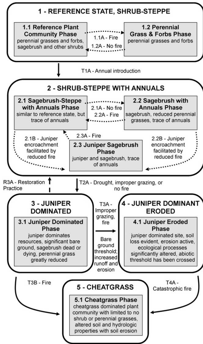
Figure 1. Example state-and-transition model (STM) showing fundamental components for the "South Slopes 12-16 PZ" Ecological Site (NRCS, 2014) located in Malheur High Plateau Mountain Land Resource Area (MLRA 23, USDA, 2006). The site includes a reference state with bluebunch wheatgrass ( Pseudoroegneria spicata [Pursh] Å. Löve ssp. spicata ), Idaho fescue ( Festuca idahoensis Elmer), Sandberg bluegrass ( Poa secunda J. Presl), and Thurber's needlegrass ( Achnatherum thurberianum [Piper] Barkworth) understory and a mountain big sagebrush ( Artemisia tridentata Nutt. subsp. vaseyana [Rydb.] Beetle), basin big sagebrush ( A. tridentata Nutt. subsp. tridentata ), and antelope bitterbrush ( Purshia tridentata [Pursh] DC.) shrub component. The site also includes alternative stable states associated with conifer encroachment by native western juniper ( Juniperus occidentalis Hook.) and invasion by the exotic annual cheatgrass ( Bromus tectorum L.) (NRCS, 2014). Individual ecological states are delineated by bold black rectangles, each with one or more within-state plant community phases (shaded rectangles). State transitions are indicated by solid black arrows. Within-state community pathways are indicated by dotted black arrows. Restoration pathways are indicated by dashed black arrows. An STM typically includes an accompanying table with text descriptions of the plant community composition, community pathway/transition dynamics, and key structural and functional indicators. See USDA (2013) and Briske et al. (2008) for detailed descriptions of components of STMs.
