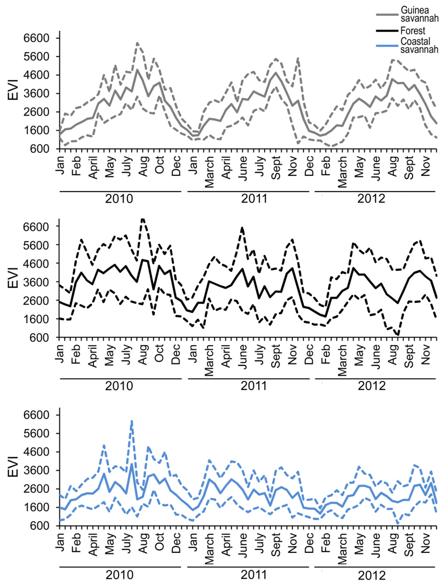
Fig 3. Enhanced Vegetation Index (EVI). EVI from 2010 through 2012 in the a) Guinea savannah, b) deciduous forest, and c) coastal savannah. EVI was extracted from MODIS satellite imagery at five sites per zone, from which mean (solid line) and \pm 1 standard deviation (dashed lines) statistics were derived.
