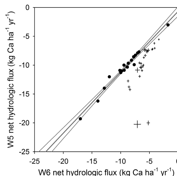
Fig. 4. Annual net hydrologic flux of Ca (kg Ca ha -1 yr -1 ) in the harvested (W5) vs. reference (W6) watersheds. Solid black circles indicate the period before the whole-tree harvest. The regression line for the preharvest period is shown, with thinner lines representing the 95% confidence intervals for the regression. Crossed bars indicate the posttreatment period with the size of the bars showing the 95% confidence intervals determined with the Monte Carlo-based uncertainty analysis.
