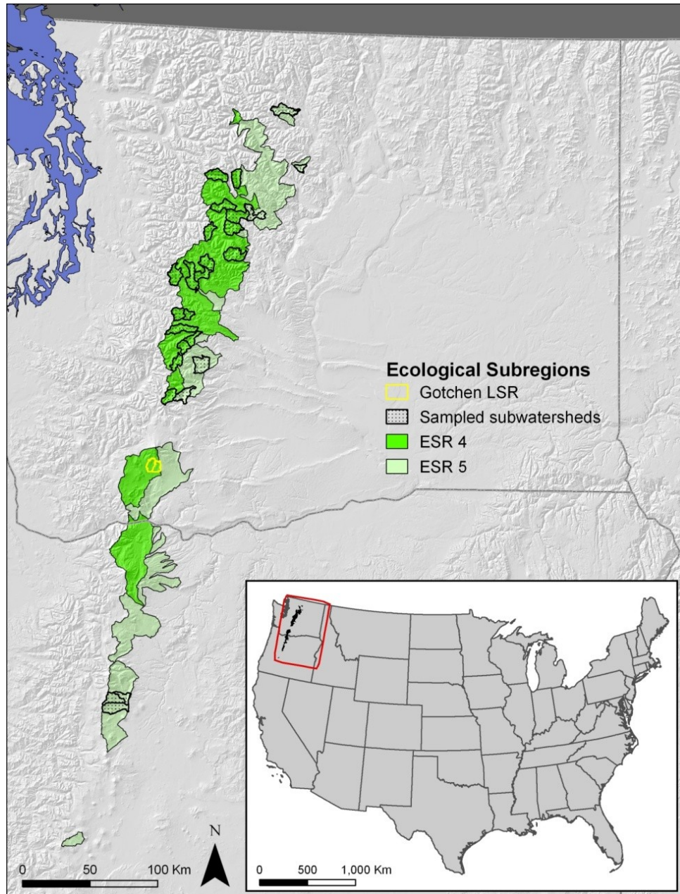
Figure S1. Location of the Gotchen Late-Successional Reserve (study area) and Ecological subregions (ESR) 4 the subregion of the study area. ESR 5 is shown as the subregion immediately to the east of ESR 4 along the west-east temperature and precipitation gradient [10] (Hessburg et al. 2000a).
