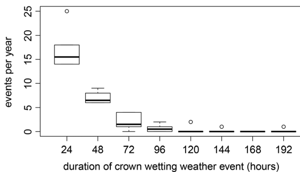
Figure 6. Box plot showing occurrence of crown wetting weather events (events per year) of different durations at Maple Creek, CA, Remote Access Weather Station from 2000 to 2005.
