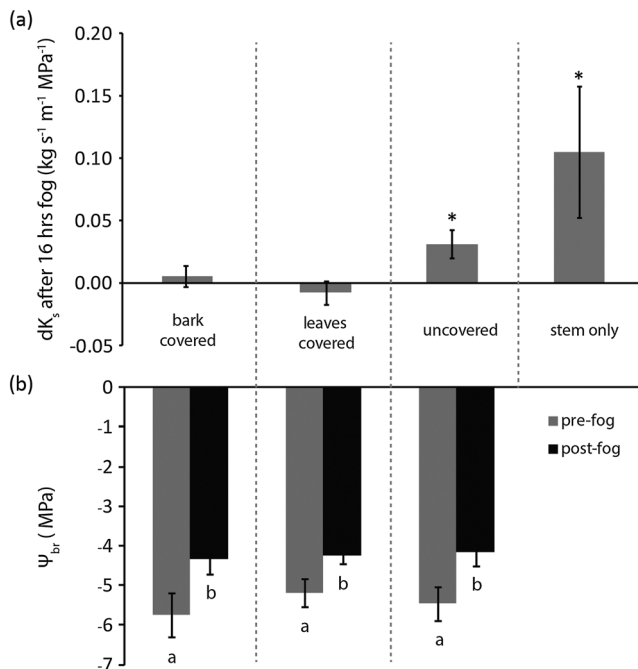
Figure 4. (a) Change in K_s after 16 h of soaking with fog with covered bark, covered leaves, uncovered bark and leaves ( n = 7 ; P < 0.05 , pairwise t -test) and stem segment only ( n = 12 , P < 0.05 , pairwise t -test). Error bars show \pm 1 standard error. (b) \Psi_{br} before and after 16 h of soaking with fog with covered bark, covered leaves and uncovered bark and leaves ( n = 7 ; P < 0.05 , Tukey HSD). Error bars show \pm 1 standard error.
