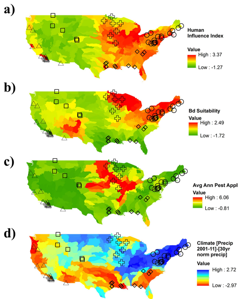
Figure 1. Spatial distribution of the four hypothesized threats to amphibian populations. Values are summarized and normalized at the HUC sub-basin scale, using ArcGIS (ver. 10.2, Redlands, CA: Environmental Systems Research Institute). (a) Human influence index. (b) Suitability for Batrachochytrium dendrobatidis . (c) Average annual pesticide application. (a–c) Red indicates higher than average threat intensity while green is lower than average. Locations of amphibian community data indicated with circles; symbols indicate region groupings (see Table 1; circles = Northeast, diamonds = Southeast, plus = Midwest, triangles = West coast, squares = Rocky Mountains). (d) The mean difference in the 30-year normal from the 2001–11 annual average precipitation; blue indicates wetter sub-basins with above average difference in precipitation while red indicates drier sub-basins.
