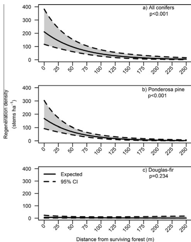
Fig. 5. Estimated (and 95% confidence interval (CI)) post-fire tree regeneration density in high severity plots as a function of distance from surviving forest, for (a) all conifers, (b) ponderosa pine, and (c) Douglas-fir.
