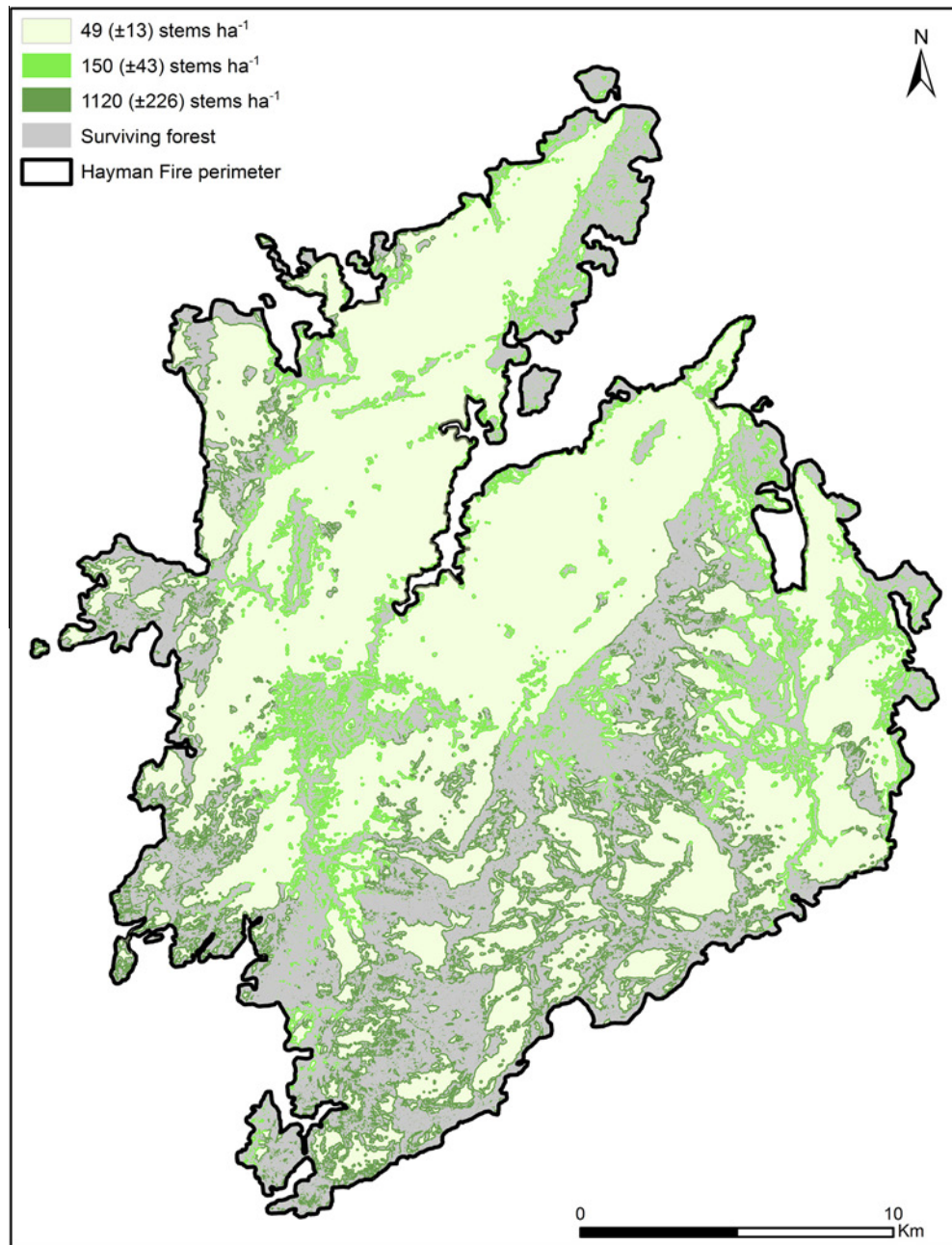
Fig. 9. Predicted mean ( \pm 1 standard error of the mean) post-fire conifer regeneration densities within unforested portions of the Hayman Fire, per the results of the all conifer regression tree analysis. Areas in pale green are \geq 50 m from surviving forest, while areas in bright green are < 50 m from surviving forest and \leq 2490 m in elevation, and areas in dark green are < 50 m from surviving forest and > 2490 m in elevation.
