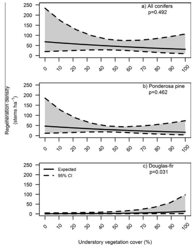
Fig. 7. Estimated (and 95% confidence interval (CI)) post-fire tree regeneration density in high severity plots as a function of understory vegetation cover for (a) all conifers, (b) ponderosa pine and (c) Douglas-fir.
