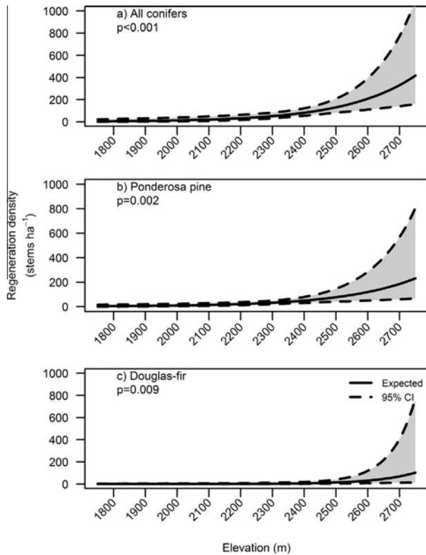
Fig. 6. Estimated (and 95% confidence interval (CI)) post-fire tree regeneration density in high severity plots as a function of elevation for (a) all conifers, (b) ponderosa pine and (c) Douglas-fir.
