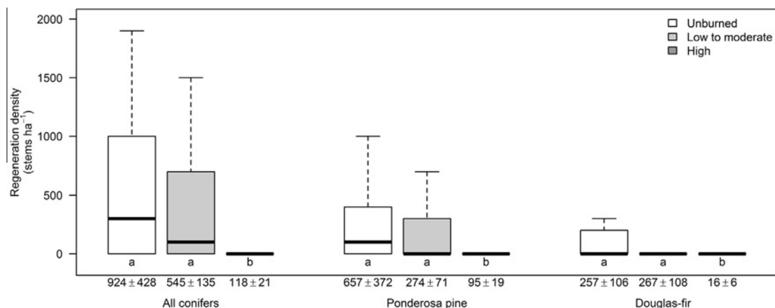
Fig. 4. Box-and-whisker diagrams depicting post-fire tree regeneration density (stems ha -1 ) by severity class and species groups. The mean ( \pm 1 standard error of the mean) density is reported along the x-axis. For each species group, fire severity classes that share letters were not significantly different ( \alpha = 0.050 ).
