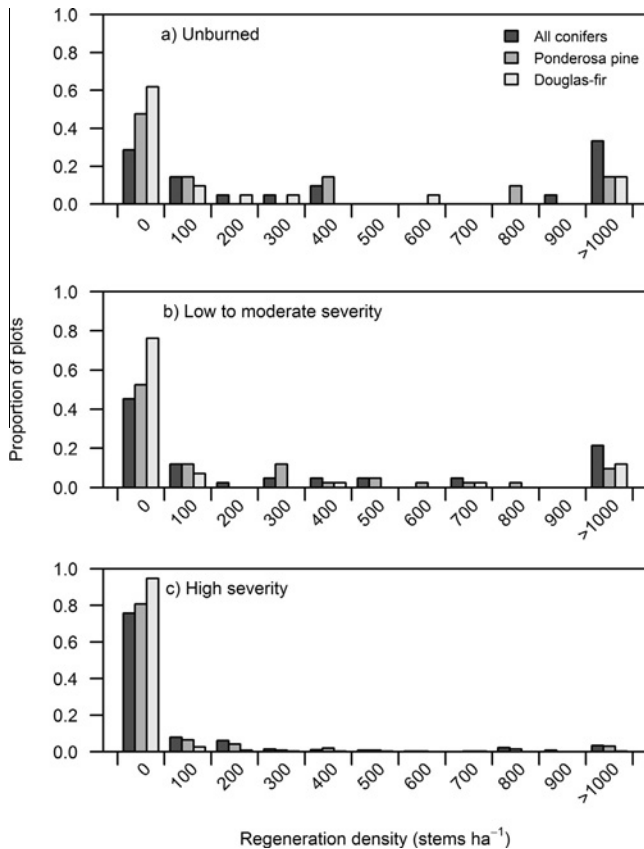
Fig. 3. Frequency distributions of post-fire tree regeneration density, by species, in (a) unburned plots, (b) low to moderate severity burn plots, and (c) high severity burn plots. Regeneration density values on the x-axis are the upper bounds of the bin.
