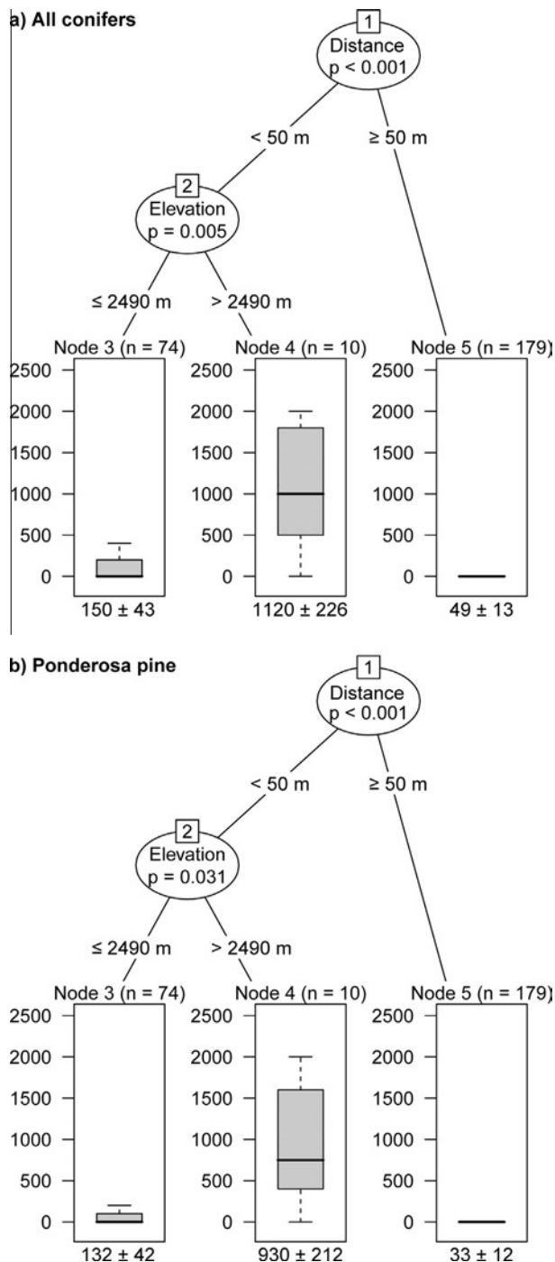
Fig. 8. Regression trees of post-fire tree regeneration density (stems \text{ha}^{-1} ) in high severity burn plots for (a) all conifers and (b) ponderosa pine. Distance is distance from surviving forest (m). Box-and-whisker diagrams are shown for each division, along with the mean ( \pm 1 standard error of the mean).
