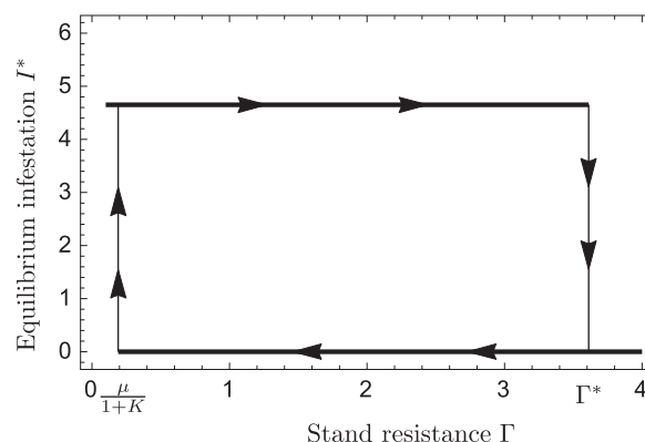
Fig. 2. Dependence of the equilibrium infestation I^* on the transformed stand resistance. This figure documents hysteresis in the forest dynamics. Untransformed parameters: g=0.001 , d=0.003 , m=0.05 , \beta_0 = 0.01 , \mu = 2000 , K=1000 . For simulations these parameters were non-dimensionalized following scheme in Table 3.
