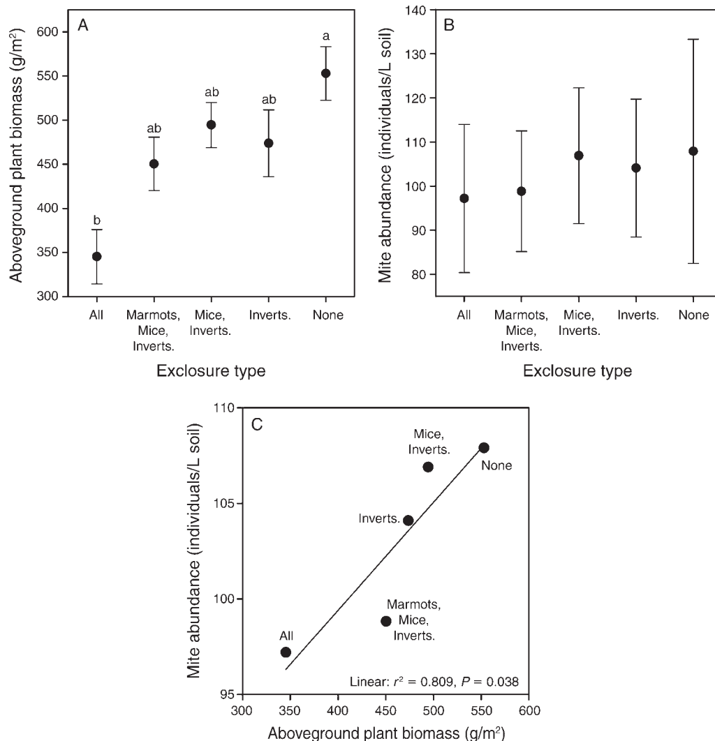
FIG. 2. Exclosure type effects on (A) aboveground plant biomass and (B) mite abundance. Values represent means \pm SE. Different lowercase letters indicate significant differences between the exclosure types ( \alpha = 0.05 ). (C) Relationship between aboveground plant biomass and mite abundance among the exclosure types. Values represent means. Exclosure types describe which aboveground herbivores are feeding on the grassland: All, all herbivores; Marmots, Mice, Inverts., medium and small mammals as well as invertebrates; Mice, Inverts., small mammals and invertebrates; Inverts., invertebrates; None, no aboveground herbivores.
