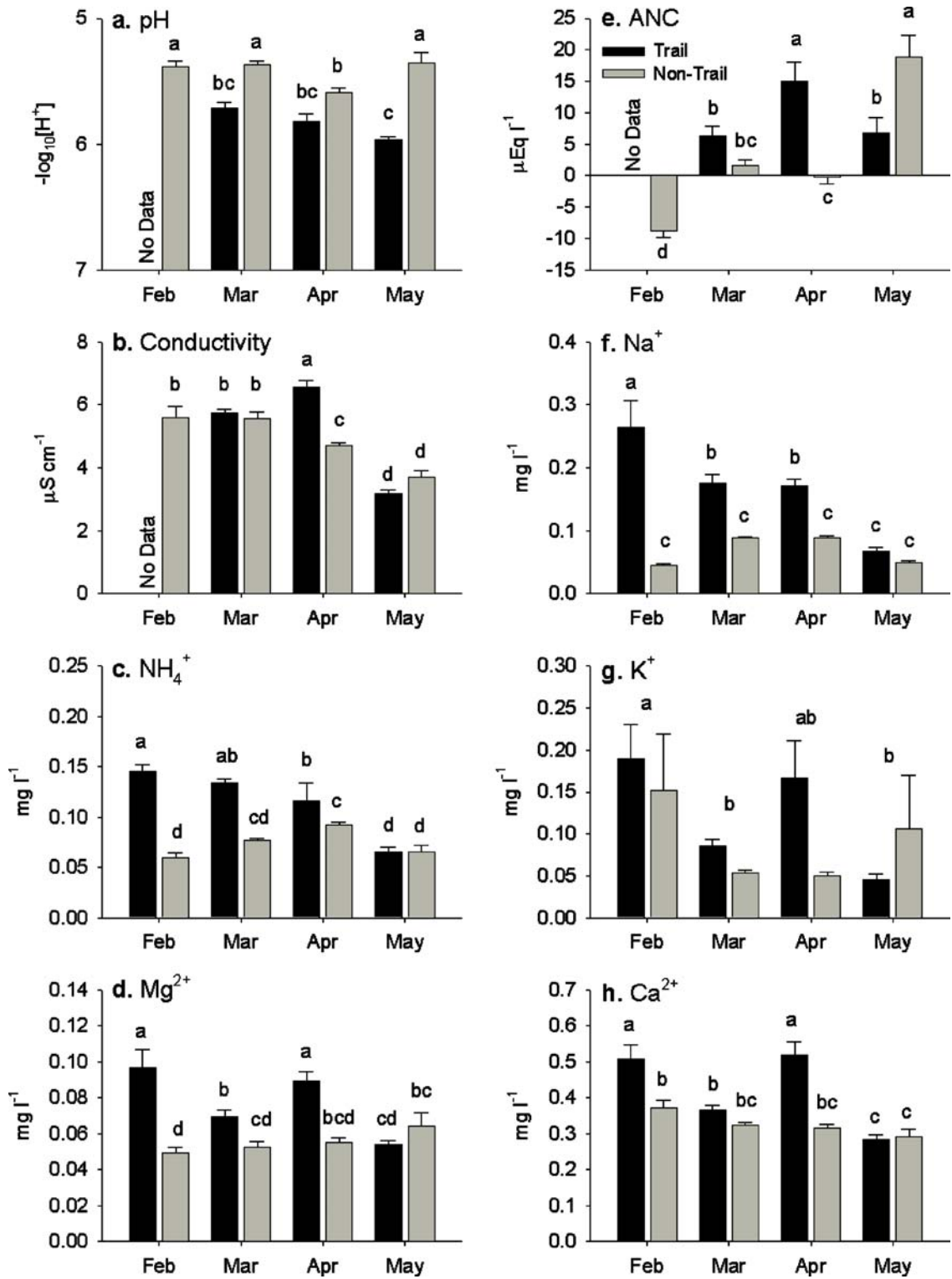
Fig. 7 pH, conductivity, and cation snow chemistry on and off the snowmobile trail, 2002. Vertical lines on each bar indicate \pm one standard error of the mean. Different letters indicate significant ( p < 0.05 ) differences
