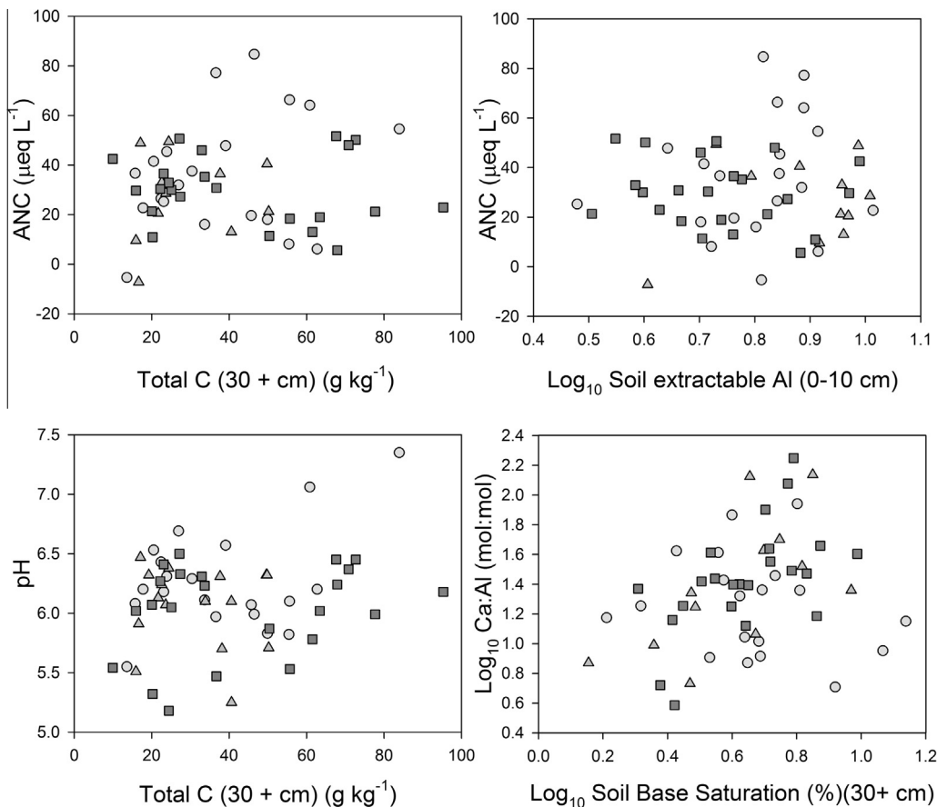
Fig. 7. Relationship between catchment mineral soil chemical characteristics that significantly inform stream chemistry variability and stream chemistry: total C concentration in the deep mineral soil and \log_{10} extractable Al in the surface mineral soil versus ANC, total C concentration in the deep mineral soil versus pH, and \log_{10} %base saturation in deep mineral soil versus \log_{10} molar Ca:Al. Data shown are mean catchment values for each watershed, North River (●), Santeetlah Creek (▲), and North Fork of the French Broad (■) for all sample dates (early summer, mid-summer, fall and spring).
