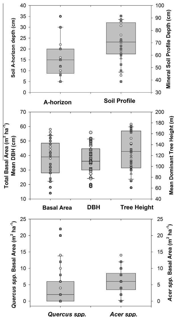
Fig. 2. Plot characterization variables were measured at each riparian and hillslope plots. A-horizon and total soil profile depth, basal area, diameter at breast height (DBH) and mean height of the 6 dominant overstory trees, and basal area of Quercus spp. and Acer spp. Plot values for each variable are shown with North River (●), Santeetlah Creek (▲), and North Fork of the French Broad (■). Box plots show watershed median value, along with the 10th, 25th, 75th and 90th percentiles.
