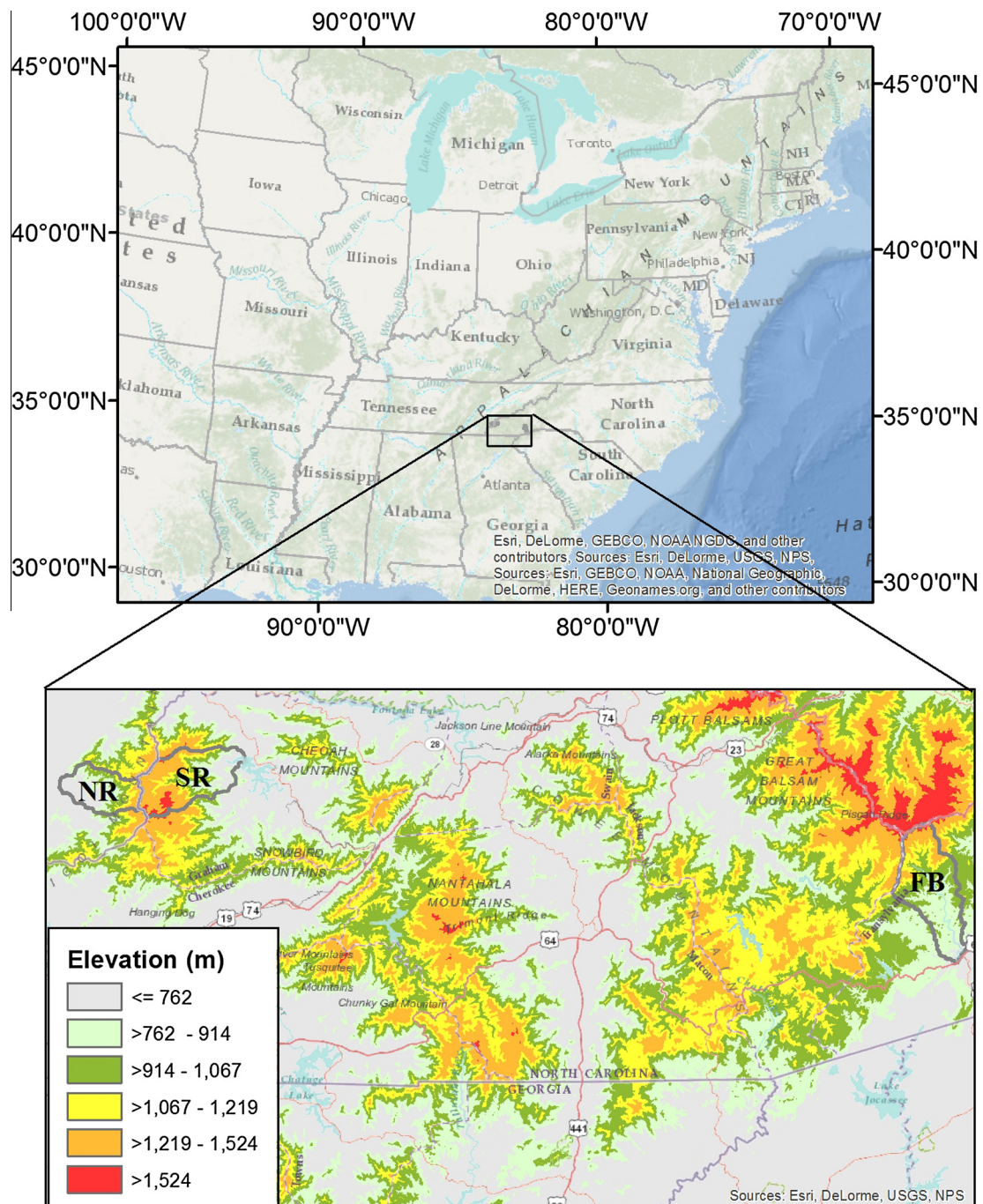
Fig. 1. Location of three watersheds sampled in this study.
