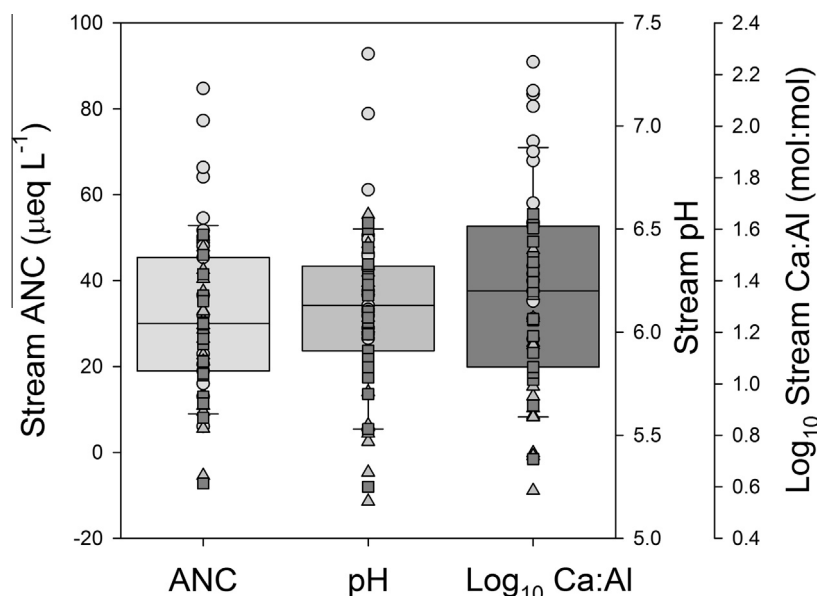
Fig. 3. Catchment stream chemistry including all sample dates (early summer, mid-summer, fall and spring) for acid neutralizing capacity (ANC), pH, and \log_{10} molar Ca:Al ratio. Shown are catchment values for each watershed, North River (●), Santeetlah Creek (▲), and North Fork of the French Broad (■). Box plots show watershed median value, along with the 10th, 25th, 75th and 90th percentiles.
