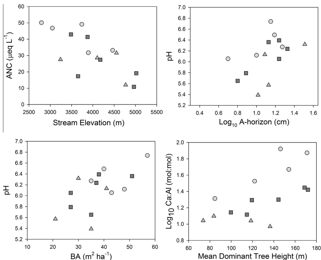
Fig. 4. Relationship between catchment non-chemical characteristics that significantly inform stream chemistry variability and stream chemistry: elevation versus ANC, \log_{10} mineral soil A-horizon depth and catchment basal area versus pH, and mean dominant tree height versus \log_{10} molar Ca:Al. Data shown are mean catchment values for each watershed, North River (●), Santeetlah Creek (▲), and North Fork of the French Broad (■).
