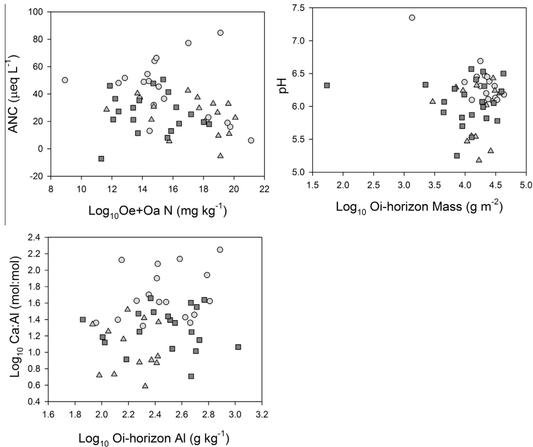
Fig. 6. Relationship between catchment O-horizon physical and chemical characteristics that significantly inform stream chemistry variability and stream chemistry: total N concentration in the Oe + Oa horizon versus ANC, \log_{10} Oi horizon mass versus pH, and \log_{10} total Al concentration in the Oi horizon versus \log_{10} molar Ca:Al. Data shown are mean catchment values for each watershed, North River (●), Santeetlah Creek (▲), and North Fork of the French Broad (■) for all sample dates (early summer, fall and spring).
