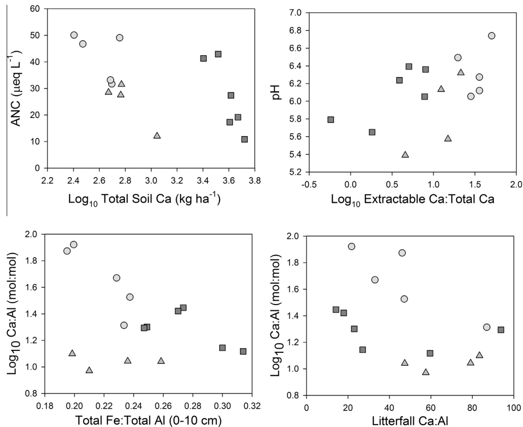
Fig. 5. Relationship between catchment geochemical characteristics that significantly inform stream chemistry variability and stream chemistry: soil profile total Ca content versus ANC, \log_{10} ratio of extractable to total Ca in surface mineral soil versus pH, and surface mineral soil Fe:Al ratio and litterfall Ca:Al versus \log_{10} molar Ca:Al. Data shown are mean catchment values for each watershed, North River (●), Santeehah Creek (▲), and North Fork of the French Broad (■).
