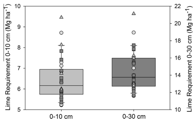
Fig. 8. Estimated lime required to increase mineral soil to pH 5.5 for the surface soil (0–10 cm) and surface plus subsurface soil (0–30 cm). Shown are plot values for each watershed, North River (●), Santeetlah Creek (▲), and North Fork of the French Broad (■). Box plots show watershed median value, along with the 10th, 25th, 75th and 90th percentiles.
