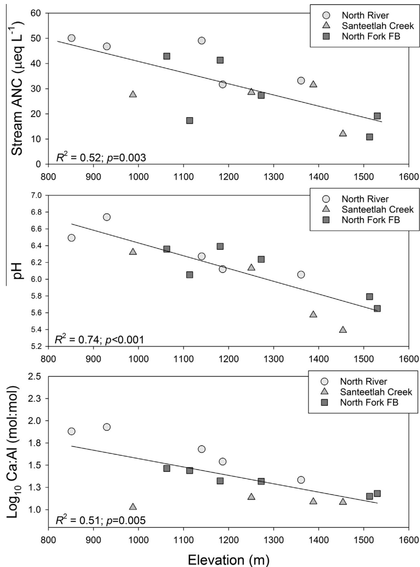
Fig. 9. Relationship between catchment stream elevation and stream chemistry: ANC, pH, and \log_{10} molar Ca:Al. Data shown are mean catchment values for each watershed, North River (●), Santeetlah Creek (▲), and North Fork of the French Broad (■).
