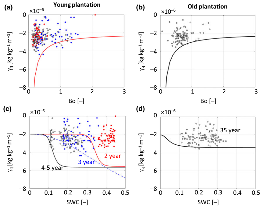
Fig. 8 Cloud formation surface ( \Delta = 0 ) compared with FA conditions, Bowen ratio (a, b) and SWC (c, d) at the Young (a, c) and Old (b, d) plantation during summertime. Colors in panels a and c refer to different stand ages as in Fig. 7.
