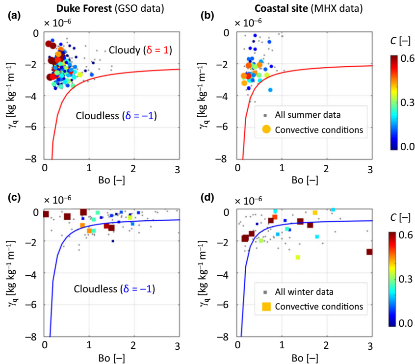
Fig. 4 Land-atmosphere conditions observed at Duke Forest and the Coastal site during summer (a, b) and winter (c, d). The solution of Eqn (9), indicating the transition from cloudy to cloudless conditions, is also shown (solid lines). Summer and winter runs with R_{n,max} = 600 \text{ W m}^{-2} and R_{n,max} = 300 \text{ W m}^{-2} , respectively, and mean summer and winter values of \gamma_0 extrapolated from Fig. 1c, e. The datasets were filtered to account for convective conditions only (see main text). All data points are shown for reference (gray dots).
