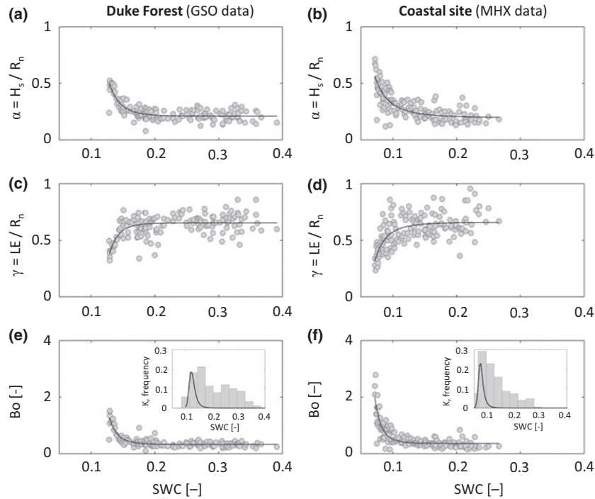
Fig. 5 Relation between surface energy fluxes (sensible heat H_s and latent heat LE normalized by net radiation R_n as in Juang et al. (2007b) and Bowen ratio Bo ) and soil water content (SWC) observed at Duke Forest (a, c, e) and the Coastal site (b, d, f). The inset in panels (e) and (f) illustrates the relative frequency of soil moisture content during the summer months (bar plot) and the curvature K of the Bo – SWC relation (black line). Curvature is defined as: K = \left| \frac{\partial^2 Bo}{\partial^2 SWC} \right| \cdot \left[ 1 + \left( \frac{\partial Bo}{\partial SWC} \right)^2 \right]^{-3/2} .
