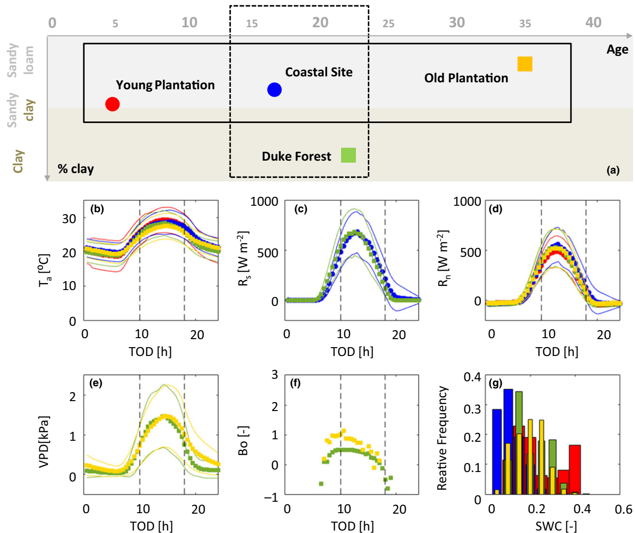
Fig. 2 Characteristics of the study sites and the interpretation of the multisite experiment: (a) soil texture, stand age, and (b–g) summertime (i.e., June–September) hydro-meteorological conditions. Temporal evolution (Time of Day, TOD) of (b) air temperature ( T_a ), (c) incoming shortwave radiation ( R_s ), (d) net radiation ( R_n ), (e) vapor pressure deficit (VPD, not available at the Coastal site/Young plantation), (f) Bowen ratio (Bo), and (g) relative frequency of soil water content (SWC) measured at the sites. In panels, b–f circles and squares represent ensemble averages for the study sites described in panel a (Coastal and Piedmont region, respectively), while solid lines are the ensemble averages \pm a standard deviation. Dotted lines in panels b–f illustrate daytime conditions as defined in this study. The Young/Old plantation are used here as a chronosequence to evaluate age-related changes in the SPA conditions while the Coastal site/Duke Forest are used to evaluate the role of edaphic conditions.
