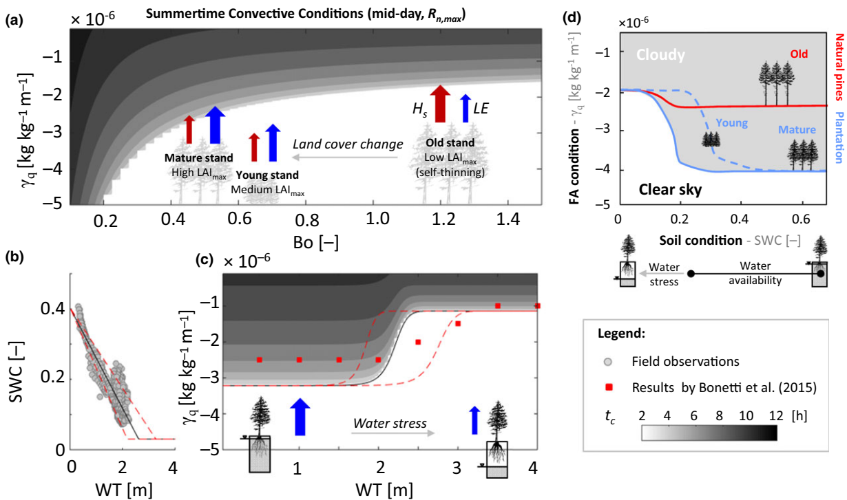
Fig. 9 Cloud formation function \Delta (continuous line) and time of cloud occurrence t_c (gray scale) as a function of (a) Bowen ratio and (c) water table depth (WT) for a given net radiation R_n ( 600 \text{ W m}^{-2} ). An empirical linear relation is used to relate WT to soil moisture content at the Coastal site (b). The approximated solution \Delta = 0 is compared with the results of numerical simulations presented in Bonetti et al. (2015) (red squares in panel c). Given the uncertainties in the WT–SWC relation, different interpolation lines have been tested (dotted lines in panels b and c). A schematic representation of age-related effects on soil–plant–atmosphere conditions regulating convective cloud formation is presented in panel d.
