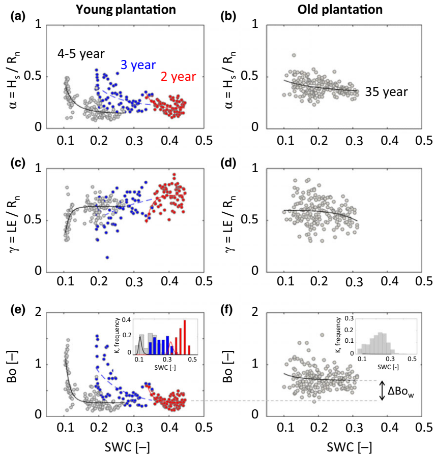
Fig. 7 Relation between surface energy fluxes and soil water content observed at the Young (a, c, e) and Old (b, d, f) plantations. The dataset from the Young plantation is divided into three subsets: year 2006 (2-year-old trees, red circles/line), year 2007 (3-year-old trees, blue circles/line), and years 2008–2009 (4- to 5-year-old trees, gray circle/black line). The inset in panels (e) and (f) illustrates the relative frequency of soil moisture content during the summer months (bar plot) and the curvature K of the Bo – SWC relation (black line).
