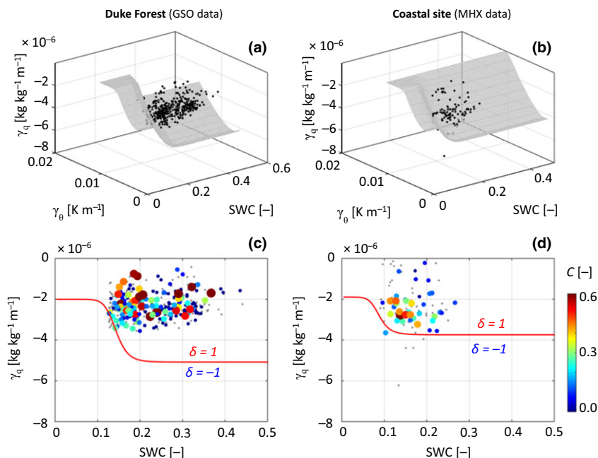
Fig. 6 Cloud formation surface ( \Delta = 0 ) compared with soil moisture and FA conditions (black dots) at Duke Forest (a) and the Coastal site (b) during summertime. In panels (c) and (d), cloudiness observed at the two sites is also shown (color bar). The transition from cloudy to cloudless conditions is illustrated by the cloud formation criterion \delta (cloudy for \delta = 1 , cloudless for \delta = -1 ). The datasets were filtered for convective conditions only (see main text). All data points are shown for reference (gray dots in panels c and d).
