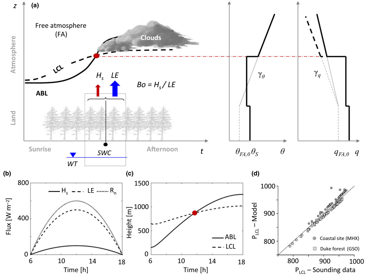
Fig. 3 Conceptual model: Soil–Plant–Atmosphere (SPA) system and potential temperature/specific humidity profiles (a). Diurnal variations of (b) latent and sensible heat fluxes for Bo = 0.2 , R_{n,max} = 600 [W m^{-2}] , \gamma_\theta = 4.0 \times 10^{-3} [K m^{-1}] , \gamma_q = -5.0 \times 10^{-6} [kg kg^{-1} m^{-1}] and (c) modeled ABL and LCL height. The ABL–LCL crossing is indicated by the dots in panel (a, d). A comparison between modeled and observed pressure at the LCL during June–July 2003 (GSO data) and 2007 (MHX data) is also shown (panel d).
