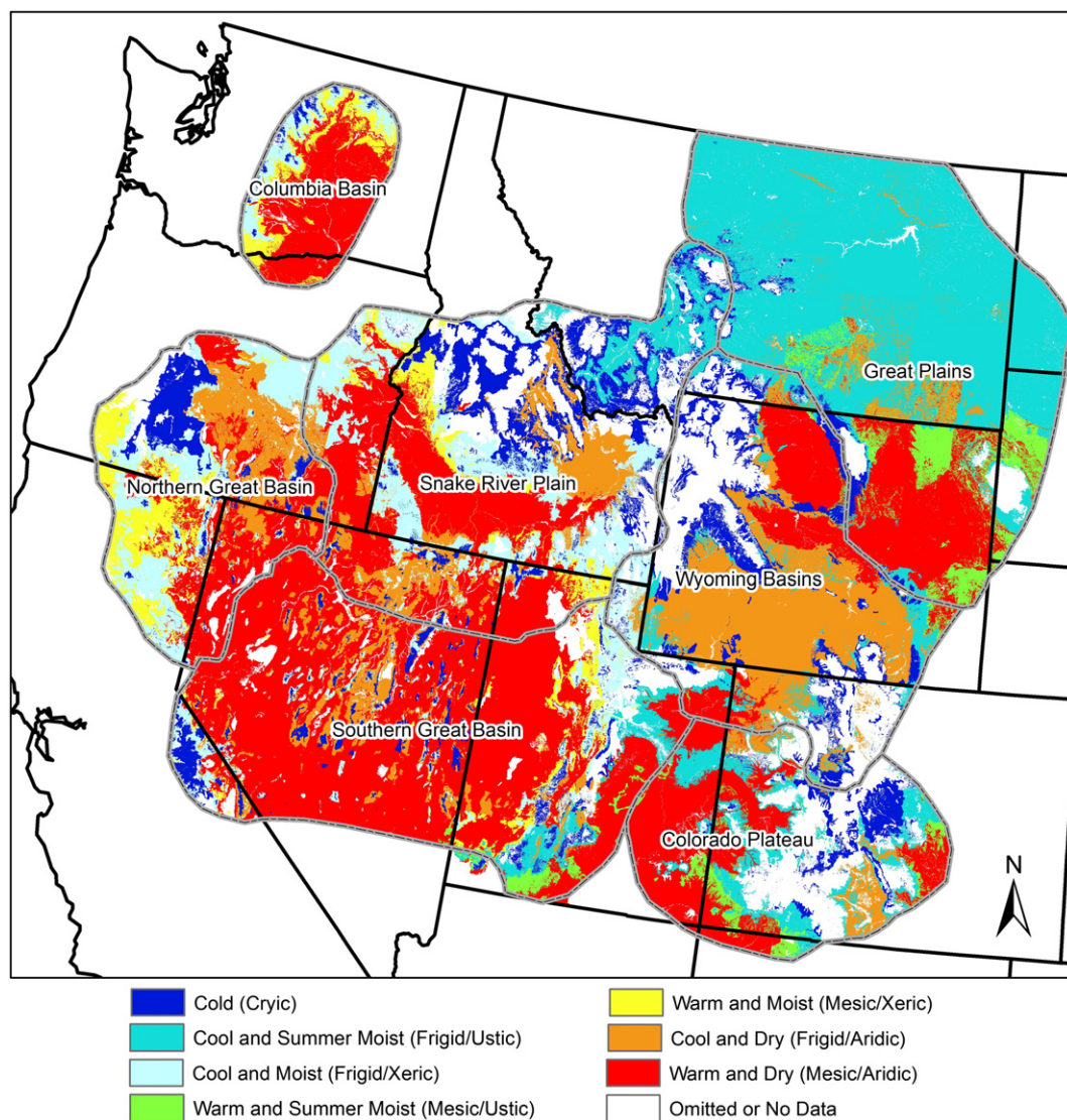
Fig. 3. Soil temperature and moisture regime classes that can be used to indicate relative ecosystem resilience and resistance across sage-grouse management zones in the western United States.
