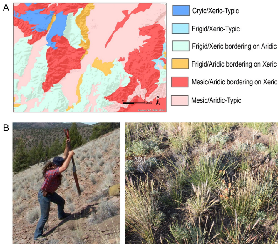
Fig. 4. Displaying soil temperature and moisture regimes down to moisture subclass (A) provides necessary refinement of the environmental gradient when evaluating potential disturbance and treatment outcomes at local scales. Maps must be combined with field verification and assessment of other site attributes that heavily influence R&R, such as, aspect, soil properties, and current vegetation (B). (Photos: NRCS).
