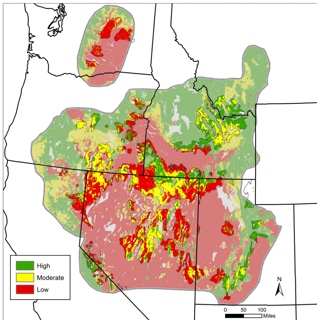
Fig. 5. Placing soil temperature and moisture regimes into simplified categories of relative R&R (high, moderate, low) provides a tool for rapid risk assessment across priority areas for sage-grouse conservation in the western range (shown here in bright colors).
