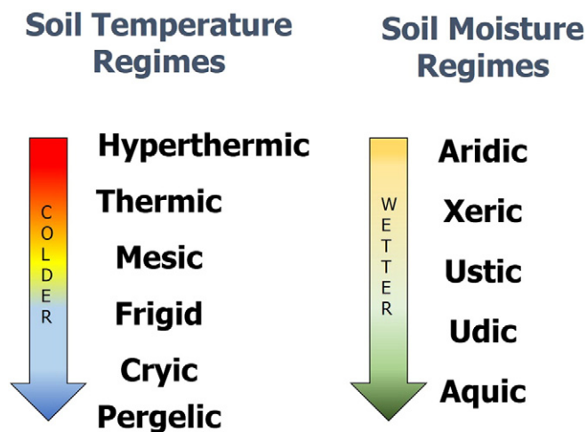
Fig. 1. Soil taxonomic temperature and moisture regime terminology. Temperature regimes are defined by specific mean soil temperatures, and seasonal fluctuations from the mean, within the main root zone. Moisture regimes relate to the length of time plant-available moisture is present during the growing season. For complete definitions see the 2014 Keys to Soil Taxonomy. 8
