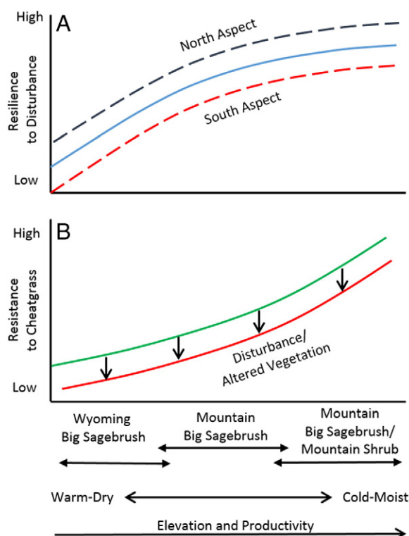
Fig. 2. Conceptual models of resilience to disturbance (A) and resistance to cheatgrass (B) over a typical soil temperature and moisture gradient in sagebrush ecosystems. 1 These relationships are modified by other soil properties, such as texture and depth, and vegetation composition and abundance. Comparing a cool and moist ( frigid/xeric ) mountain big sagebrush site in Nevada (C) to a warm and dry ( mesic/aridic ) Wyoming big sagebrush site in Oregon (D) illustrates broad differences in site productivity across sagebrush ecosystems that are correlated with potential resilience and resistance (Photos: Richard F. Miller, Jeanne C. Chambers).
