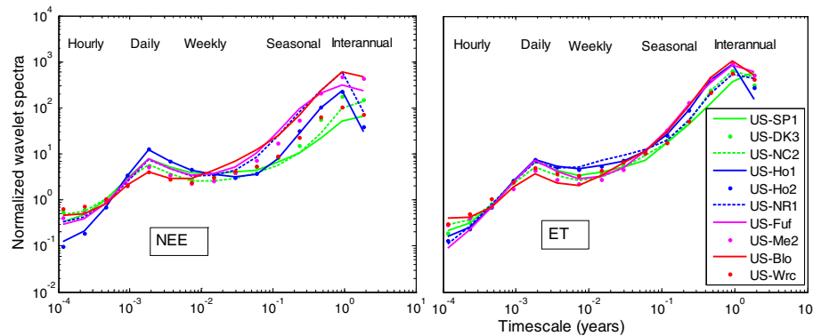
Fig. 4 Normalized wavelet spectra of net ecosystem \text{CO}_2 exchange (NEE, \mu\text{mol m}^{-2} \text{s}^{-1} ) and evapotranspiration (ET, \text{mm } 30\text{-min}^{-1} ) at ten forest sites. Half-hourly data were used in the analysis
