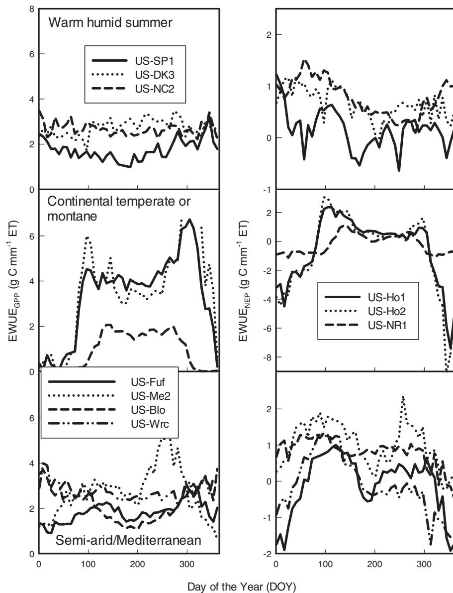
Fig. 3 Seasonal changes (8-day averages) of ecosystem water use efficiency ( EWUE_{GPP} and EWUE_{NEP} ) based on gross primary production (GPP) and evapotranspiration (ET) and net ecosystem production (NEP) and ET at ten forest sites, respectively
