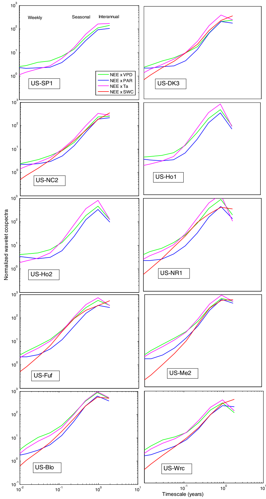
Fig. 6 Normalized wavelet cospectra between net ecosystem \text{CO}_2 exchange ( NEE ) and major climate variables (vapor pressure deficit ( VPD ), photosynthetically active radiation ( PAR ), air temperature ( T_a ), and soil water content ( SWC )) at ten forest sites. Half-hourly data were used in the analysis. SWC data were not available in some sites
