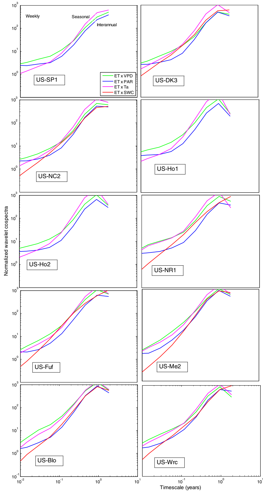
Fig. 7 Normalized wavelet cospectra between evapotranspiration ( ET ) and major climate variables (vapor pressure deficit ( VPD ), photosynthetically active radiation ( PAR ), air temperature ( T_a ), and soil water content ( SWC )) at ten forest sites. Half-hourly data were used in the analysis. SWC data were not available in some sites
