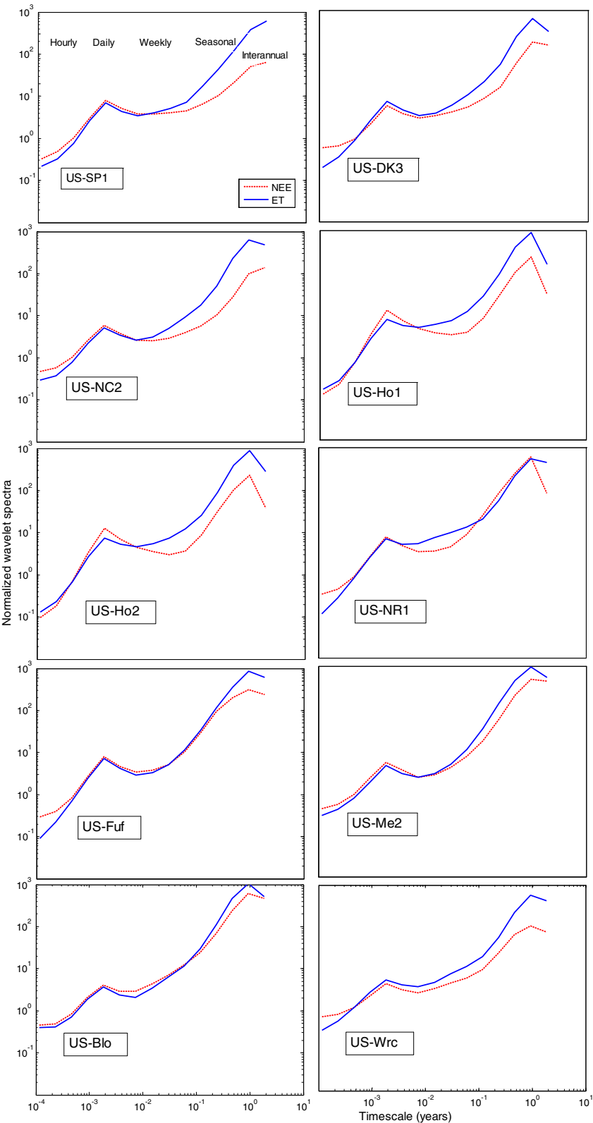
Fig. 5 A comparison of the normalized wavelet spectra of net ecosystem CO 2 exchange (NEE, \mu\text{mol m}^{-2} \text{s}^{-1} ) and evapotranspiration (ET, \text{mm 30-min}^{-1} ) at each forest site. Half-hourly data were used in the analysis
