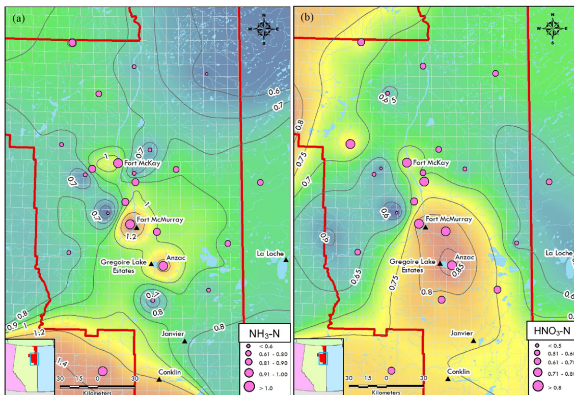
Fig. 4. Four-year annual average dry deposition from 2009 to 2012 in the AOSR in \text{kg N ha}^{-1} \text{ yr}^{-1} for (a) \text{NH}_3\text{-N} ; (b) \text{HNO}_3\text{-N} ; (c) \text{NO}_2\text{-N} ; (d) total N ( \text{N}_t ); and (e) \text{SO}_2\text{-S} ( \text{kg ha}^{-1} \text{ yr}^{-1} ).
