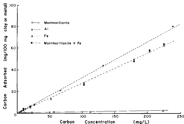
FIG. 2. Adsorption of DOC from alder leachate by amorphous precipitates of Fe and Al and a montmorillonitic clay saturated with Fe. The adsorption by montmorillonitic clay saturated with sodium from the previous figure is shown for reference.
