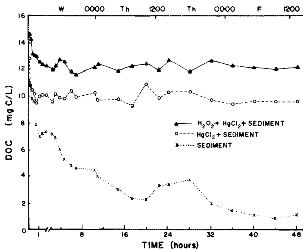
FIG. 4. Concentration of DOC in each recirculating chamber throughout period when radiocarbon uptake was measured. A concentration increase in DOC of 9.8 mg C/L was initially added to each chamber by the alder leachate. Differences in initial concentration of DOC in each chamber resulted from unequal background levels of DOC.
