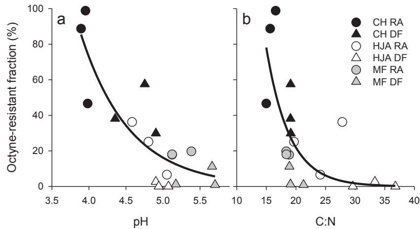
Fig. 4. Relationship between the octyne-resistant (AOA) fraction of nitrification in whole soil supplemented with \text{NH}_3 (equivalent to 140 \text{ mg NH}_4^+\text{-N kg}^{-1} soil) and soil pH (a) and C:N ratio (b). Soils are identified by site (CH—Cascade Head, black; HJA—H.J. Andrews, white; MF—McDonald Forest, gray) and tree type (DF—Douglas-fir, triangle; RA—red alder, circle). Lines represent best fit, exponential regressions; all are significant at p < 0.05 .
