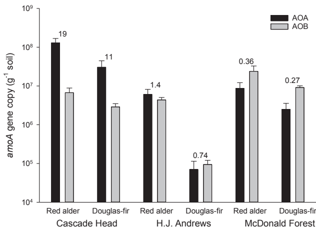
Fig. 5. Abundance of ammonia-oxidizing archaea (AOA) and bacteria (AOB) based on copy numbers of their amoA genes. Data are means \pm standard error ( n = 3 ). Number above a set of bars is the AOA:AOB ratio.
