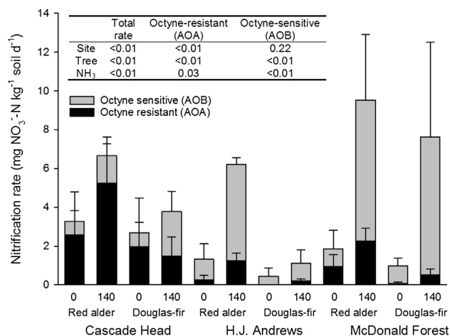
Fig. 3. Nitrification activities of octyne-resistant (archaeal) and octyne-sensitive (bacterial) ammonia oxidizers in whole soil assays supplemented with \text{NH}_3 equivalent to 0 or 140 \text{mg NH}_4\text{-N kg}^{-1} soil. Data are means \pm standard errors ( n = 3 ). Three-way ANOVA table shows the statistical significance ( p -value) of site, tree type, and \text{NH}_3 addition; interactions were not significant ( p > 0.05 ).
