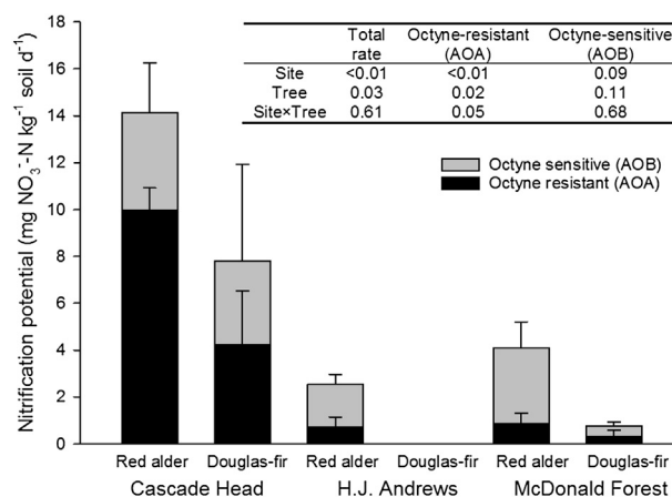
Fig. 1. Potential nitrification activities of octyne-resistant (archaeal) and octyne-sensitive (bacterial) ammonia oxidizers in short-term soil slurry assays supplemented with 1 mM NH 4 + (~140 mg NH 4 + N kg -1 soil). Data are means \pm standard errors ( n = 3 ). No potential nitrification activity was found for the Douglas-fir soil at the H.J. Andrews. Two-way ANOVA table shows the statistical significance ( p -value) of site, tree type, and their interaction.
