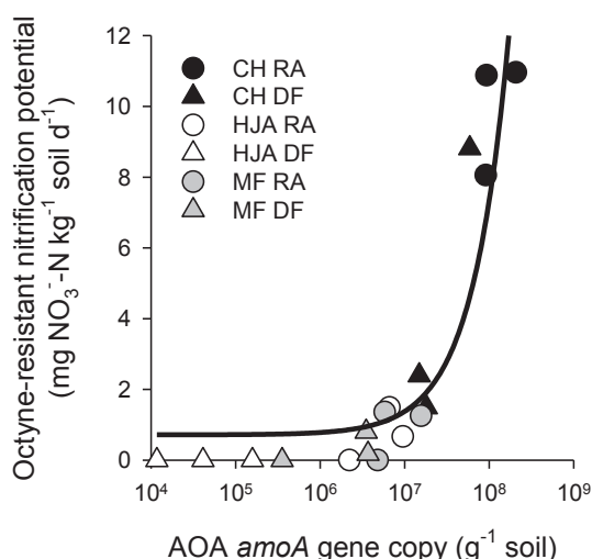
Fig. 7. The rate of octyne-resistant (AOA) nitrification potential is strongly correlated with AOA amoA gene copy numbers. Soils are identified by site (CH—Cascade Head, black; HJA—H.J. Andrews, white; MF—McDonald Forest, gray) and tree type (DF—Douglas-fir, triangle; RA—red alder, circle). Line represents exponential regression ( R^2 = 0.80 , p < 0.01 ).
