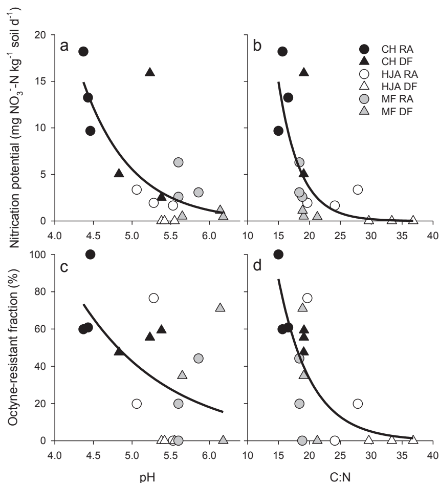
Fig. 2. Relationship between total nitrification potential (a, b) or octyne-resistant (AOA) fraction of the nitrification potential (c, d) and soil slurry pH (a, c) and C:N ratio (b, d). Soils are identified by site (CH—Cascade Head, black; HJA—H.J. Andrews, white; MF—McDonald Forest, gray) and tree type (DF—Douglas-fir, triangle; RA—red alder, circle). Lines represent best fit, exponential regressions; all are significant at p < 0.05 .
