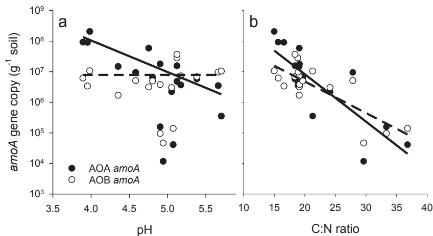
Fig. 6. Relationship between ammonia-oxidizing archaea (AOA) or bacteria (AOB), based on copy numbers of their amoA genes, and soil pH (a) and C:N ratio (b). Copy numbers of AOA amoA genes (black circles, solid lines) were significantly correlated with soil pH ( R^2 = 0.32 , p = 0.01 ) and C:N ratio ( R^2 = 0.68 , p < 0.01 ), whereas AOB amoA gene copy numbers (white circles, dashed lines) were correlated with only soil C:N ratio ( R^2 = 0.63 , p < 0.01 ) but not pH ( p = 0.81 ).
