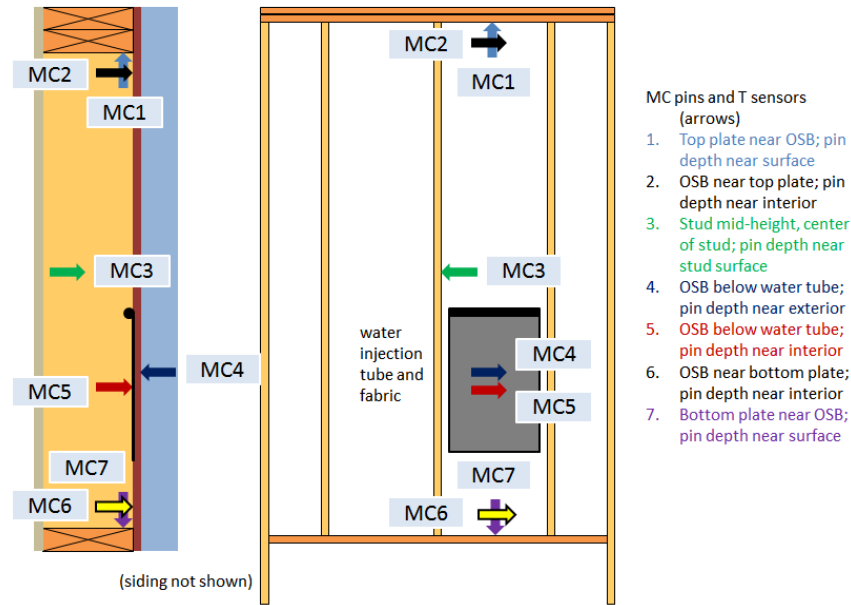
Figure 3. Placement of moisture content/temperature sensors
