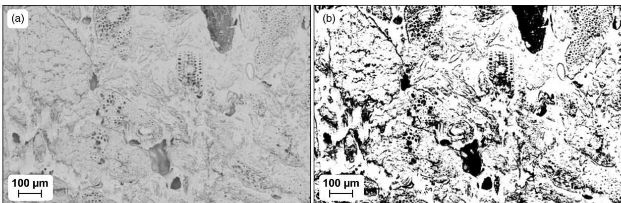
Figure 12. Example of (a) SEM image and (b) corresponding processed image used to determine the void content.
