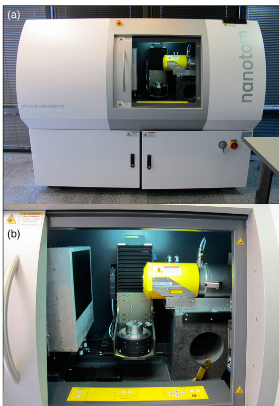
Figure 2. GE phoenix X-ray nanotom m used in the CT evaluation.
