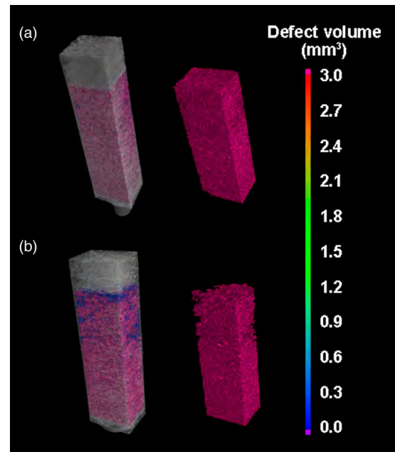
Figure 7. MicroCT images (14 \mu\text{m} voxel size) of field-exposed samples showing the 3D reconstructed volume containing all detected voids (left) and a 3D isolation of the largest detected void (right) for the (a) Shadow and (b) Sun samples.
