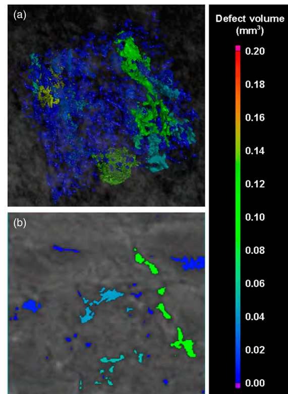
Figure 8. MicroCT images (20 \mu\text{m} voxel size) of a Reference sample showing (a) a 3D reconstructed sub-volume and (b) a corresponding 2D slice from this sub-volume.
