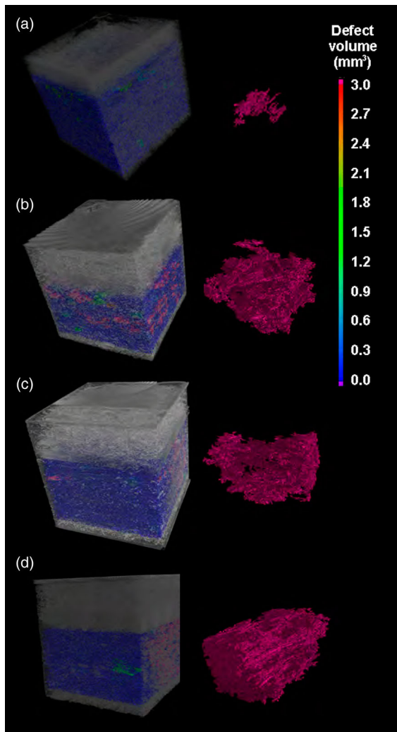
Figure 6. MicroCT images (14 \mu\text{m} voxel size) of laboratory soil block samples showing the 3D reconstructed volume containing all detected voids (left) and a 3D isolation of the largest detected void (right) for samples at the following test conditions: (a) no conditioning, no fungal exposure, (b) conditioned, no fungal exposure, (c) no conditioning, white-rot exposure, (d) conditioned, white-rot exposure.
