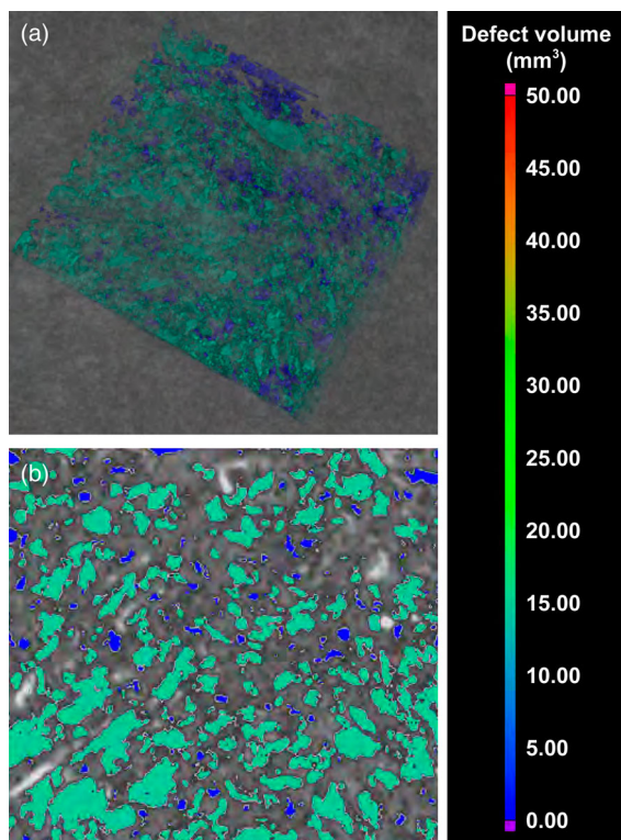
Figure 9. MicroCT images (20 \mu\text{m} voxel size) of a Shadow sample showing (a) a 3D reconstructed sub-volume and (b) a corresponding 2D slice from this sub-volume.
