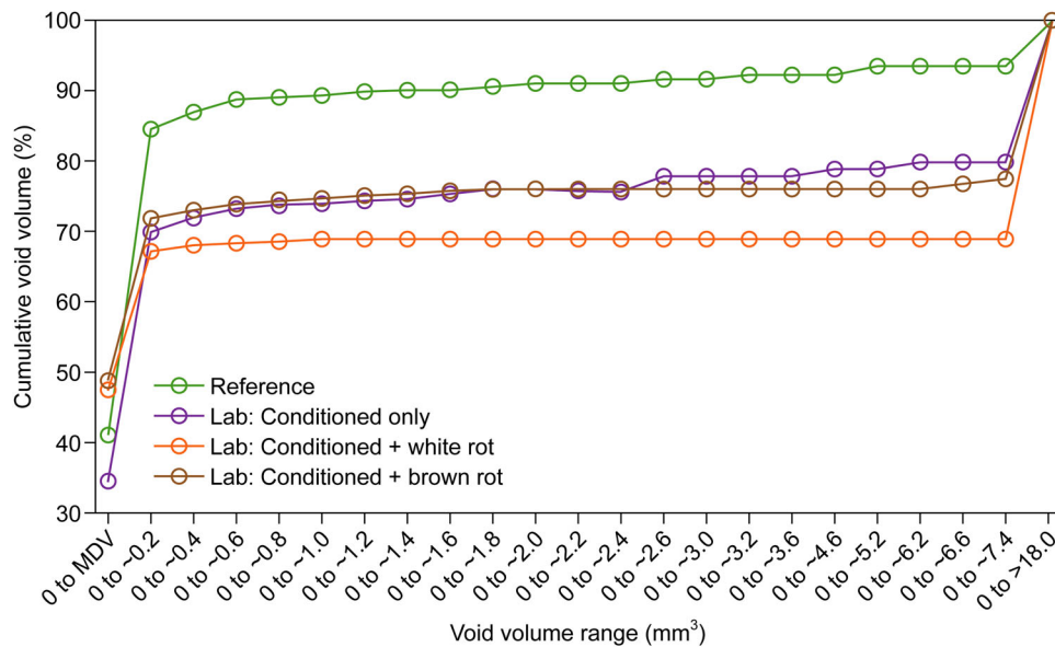
Figure 11. Line graph showing the cumulative distribution of detected voids based on the total void volume for Reference and select laboratory-exposed samples; MDV here stands for minimum detected volume which is 2.7 \times 10^{-6} \text{ mm}^3 at the 14 \mu\text{m} voxel size.
