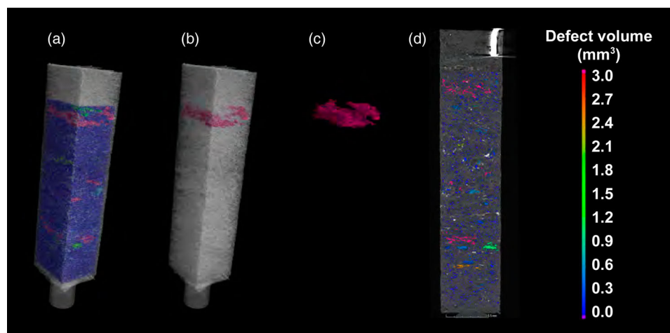
Figure 5. MicroCT images (14 \mu\text{m} voxel size) of Reference-3 sample showing (a) 3D reconstructed volume containing all detected voids, (b) 3D reconstructed volume containing only the largest detected void, (c) 3D isolation of the largest detected void, and (d) 2D slice obtained at the center of the sample.
