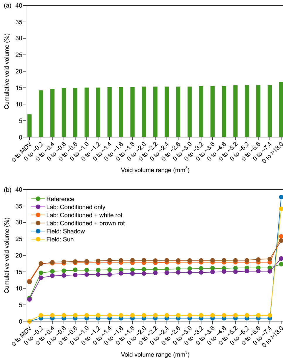
Figure 10. (a) Histogram showing the cumulative distribution of detected voids based on the total analyzed volume for the Reference sample, and (b) corresponding line graph showing the cumulative distribution of detected voids for the Reference sample and select laboratory- and field-exposed samples; MDV here stands for minimum detected volume which is 2.7 \times 10^{-6} \text{ mm}^3 at the 14 \mu\text{m} voxel size.
