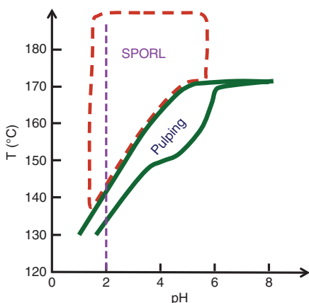
Figure 1: Comparison of operating conditions between SPORL and sulfite pulping in the temperature–pH diagram.
