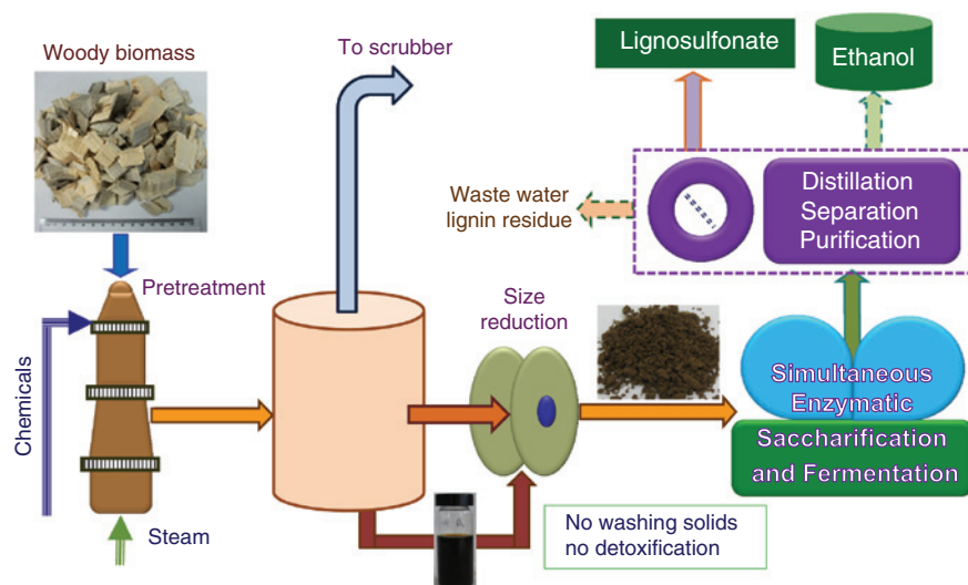
Figure 2: A schematic diagram shows the process flow of scale-up pretreatment of BKLP by SPORL and downstream saccharification and fermentation. Process boxed by dashed lines was partially conducted.
