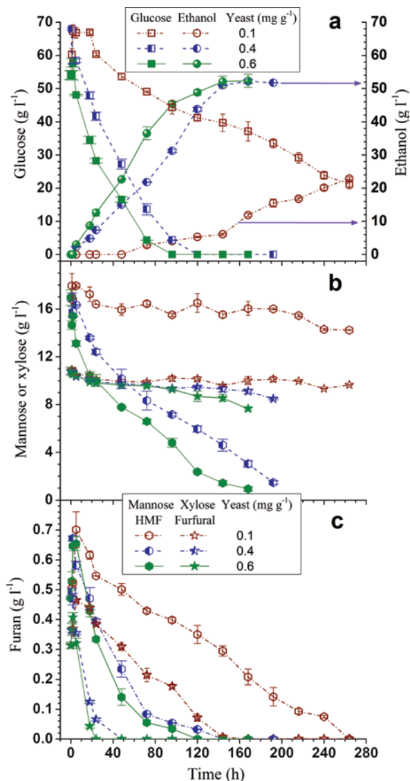
Figure 4: Time-dependent sugar, ethanol, and furan concentration profiles in the fermentation broth using the whole biomass slurry from the scale-up SPORL pretreatment at 20% total solids loading. (a) glucose and ethanol (b) mannose and xylose (c) furans.
