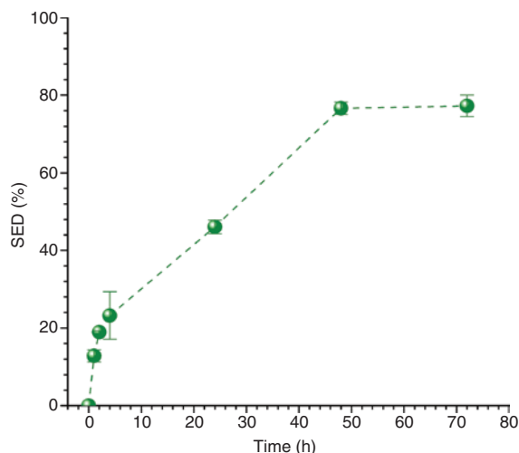
Figure 3: Time-dependent enzymatic saccharification efficiency of washed solids of BKLP pretreated by SPORL at pilot-scale at a low CTec3 loading of 10 FPU/g glucan.
