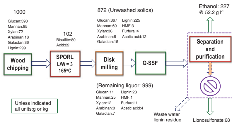
Figure 5: A block diagram shows process mass balance for the pilot-scale pretreatment of BKLP with subsequent saccharification and fermentation. Process boxed by dashed lines was partially conducted.
