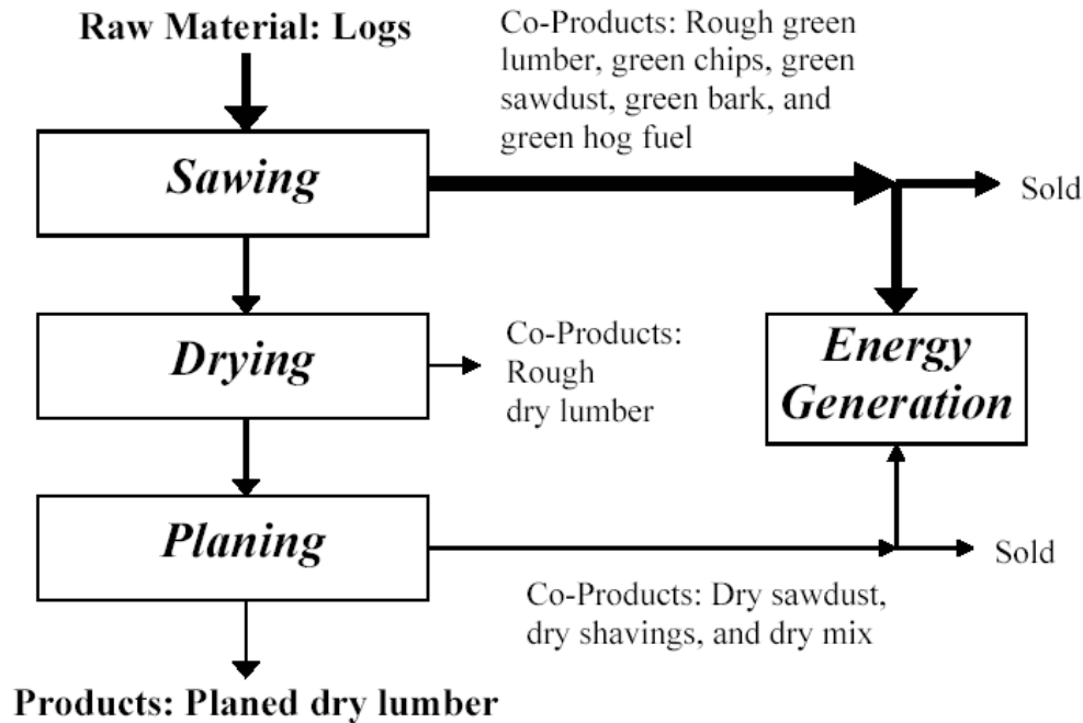
Figure 2.1. Description of the four unit processes for hardwood lumber manufacturing showing material flow.
