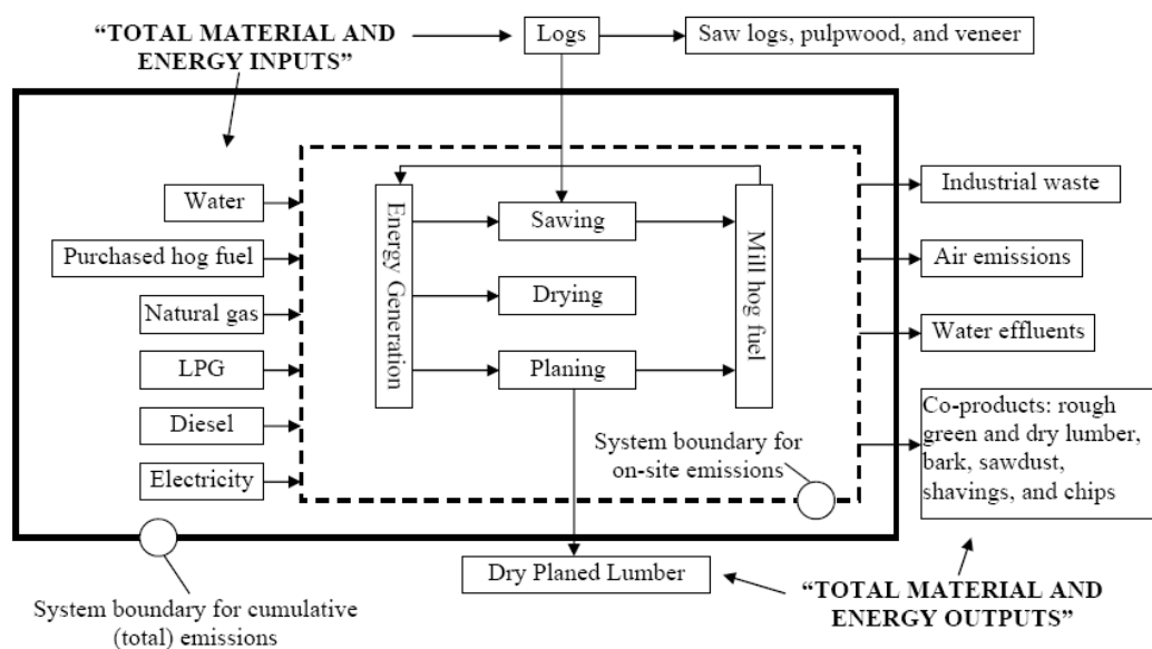
Figure 2.2. System boundaries for hardwood lumber production
