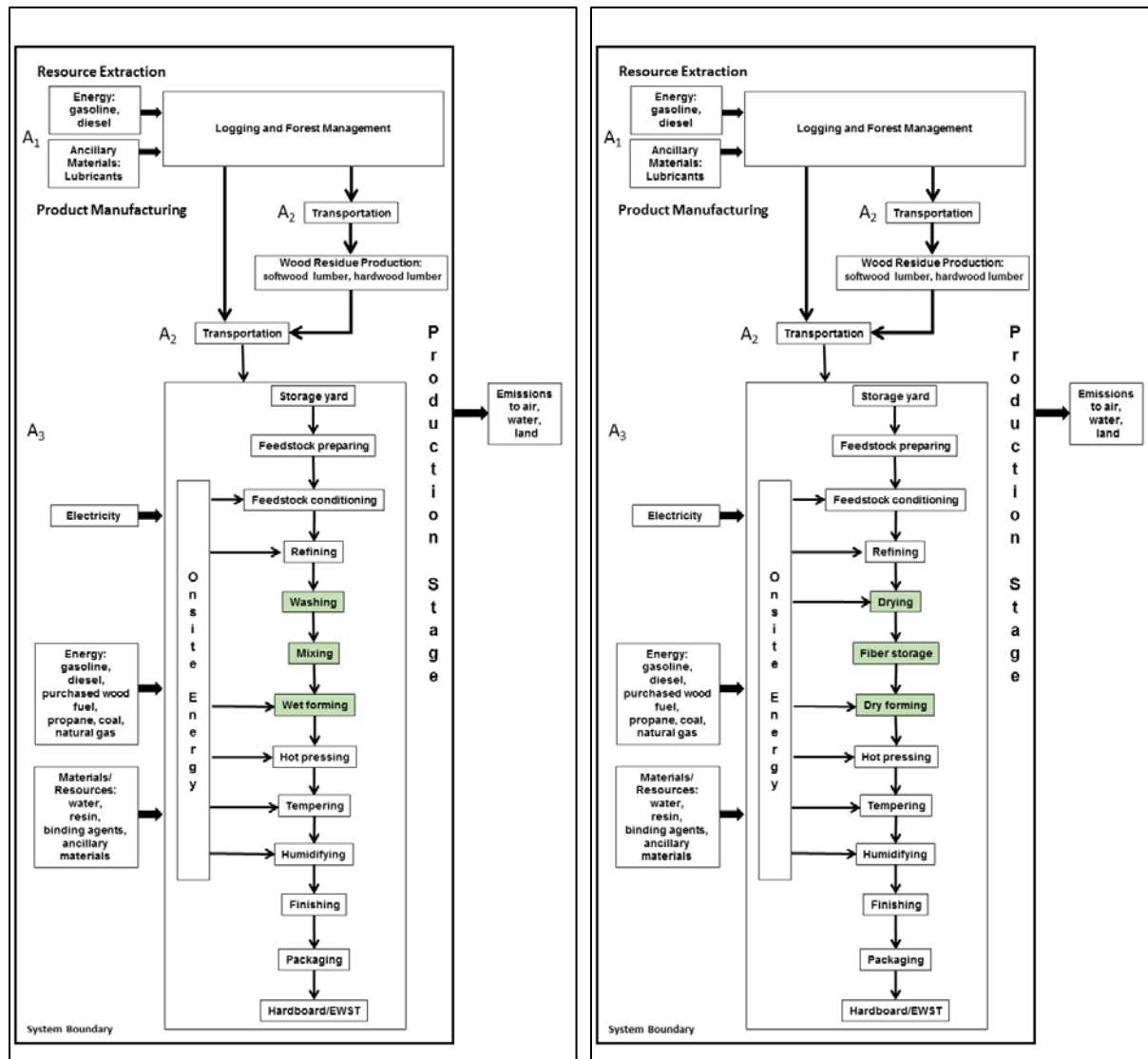
Figure 6. System boundary and process flow for cradle-to-gate production of hardboard for both wet and dry forming processes.
